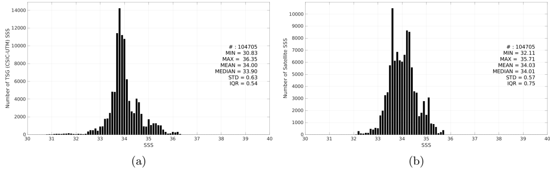
Figure 3: Histograms of SSS from TSG (CSIC-UTM) (a) and SMOS SSS L3 v332 - 9 Days (CATDS-CPDC) (b) considering all match-up pairs per bins of 0.1 over the Roaring Forties and Furious Fifties Pi-MEP region and for the full satellite product period.
