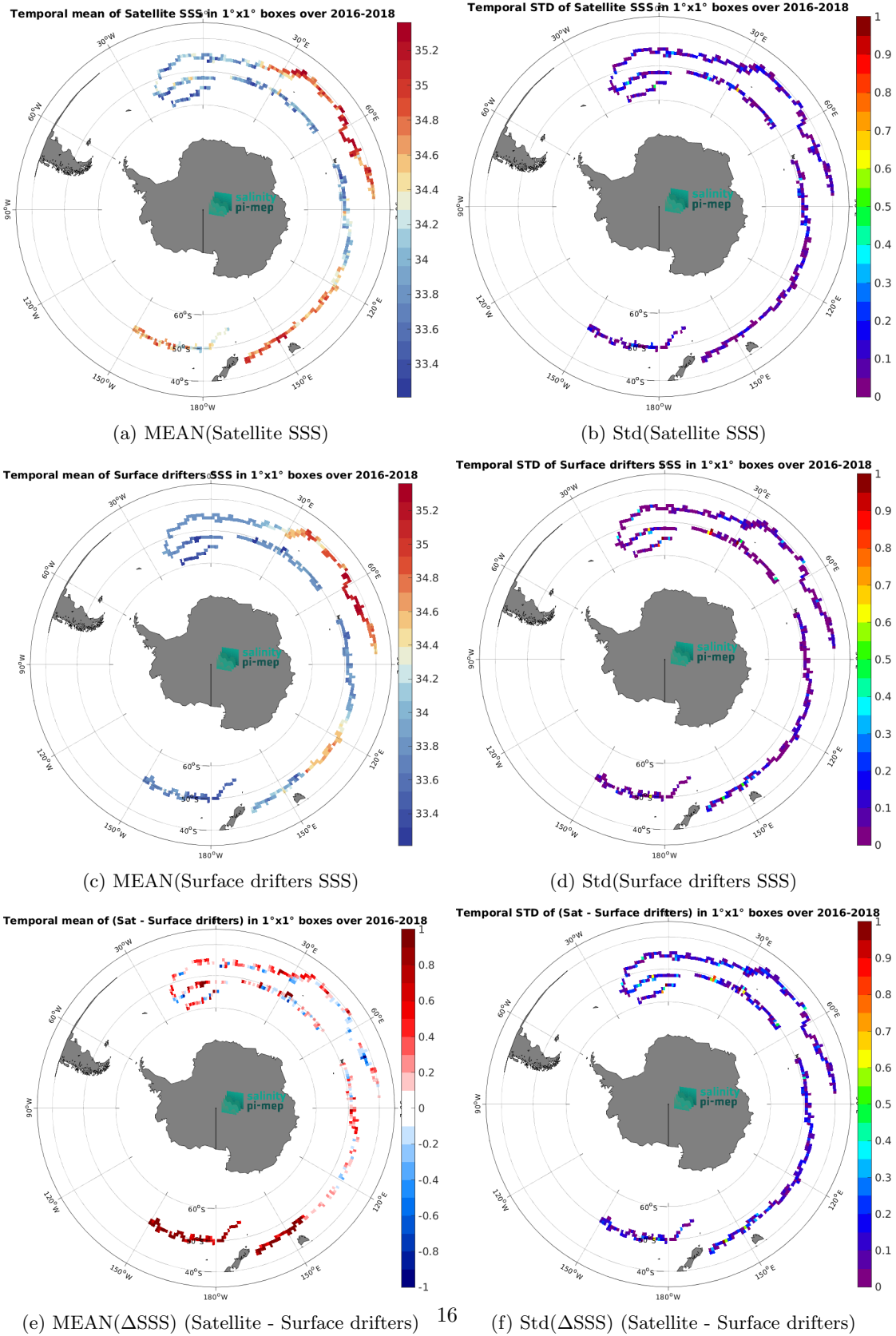
Figure 6: Temporal mean (left) and Std (right) of SSS from SMOS SSS L3 v332 - 9 Days (CATDS-CPDC) (top), Surface drifters (middle), and of \Delta SSS (Satellite - Surface drifters). Only match-up pairs are used to generate these maps.
