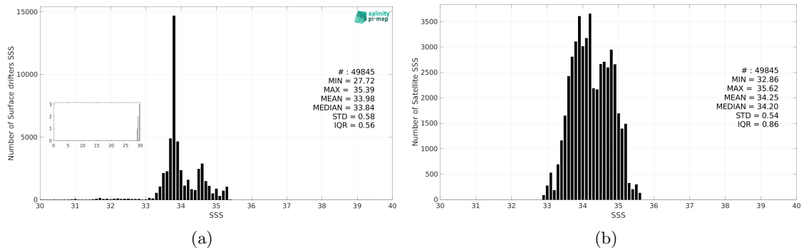
Figure 3: Histograms of SSS from Surface drifters (a) and SMOS SSS L3 v332 - 9 Days (CATDS-CPDC) (b) considering all match-up pairs per bins of 0.1 over the Roaring Forties and Furious Fifties Pi-MEP region and for the full satellite product period.
