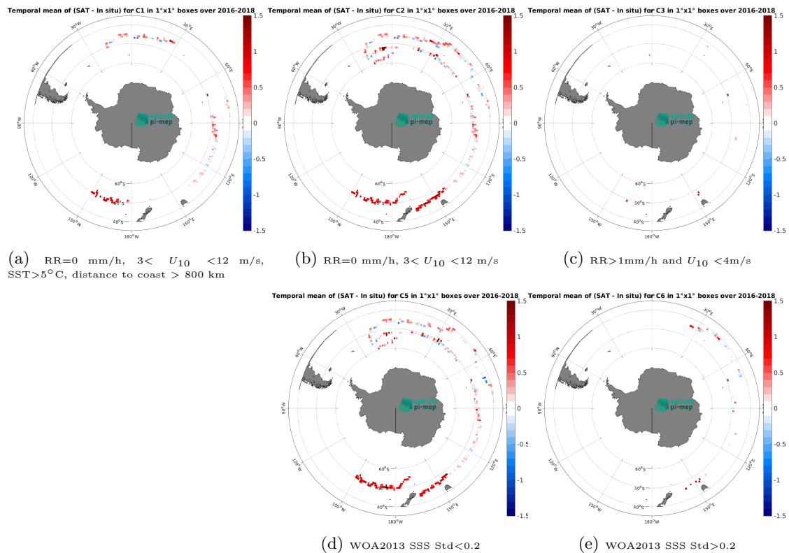
Figure 13: Temporal mean gridded over spatial boxes of size 1^\circ \times 1^\circ of \Delta SSS (SMOS SSS L3 v332 - 9 Days (CATDS-CPDC) - Surface drifters) for 5 different subdatasets corresponding to:RR=0 mm/h, 3 < U_{10} < 12 m/s, SST >5^\circ\text{C} , distance to coast > 800 km (a), RR=0 mm/h, 3 < U_{10} < 12 m/s (b), RR >1 mm/h and U_{10} < 4 m/s (c), WOA2013 SSS Std <0.2 (d), WOA2013 SSS Std >0.2 (e).
