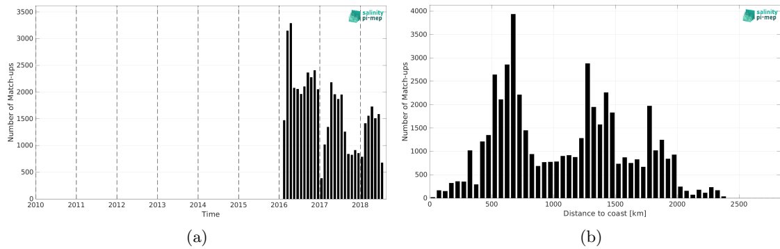
Figure 2: Number of match-ups between Surface drifters and SMOS SSS L3 v332 - 9 Days (CATDS-CPDC) SSS as a function of time (a) and as function of the distance to coast (b) over the Roaring Forties and Furious Fifties Pi-MEP region and for the full satellite product period.
