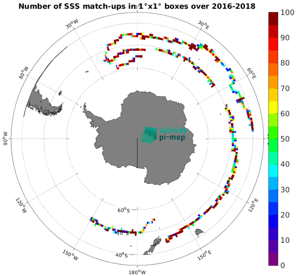
Figure 4: Number of SSS match-ups between Surface drifters SSS and the SMOS SSS L3 v332 - 9 Days (CATDS-CPDC) SSS product for the Roaring Forties and Furious Fifties Pi-MEP region over 1^\circ \times 1^\circ boxes and for the full satellite product period.
