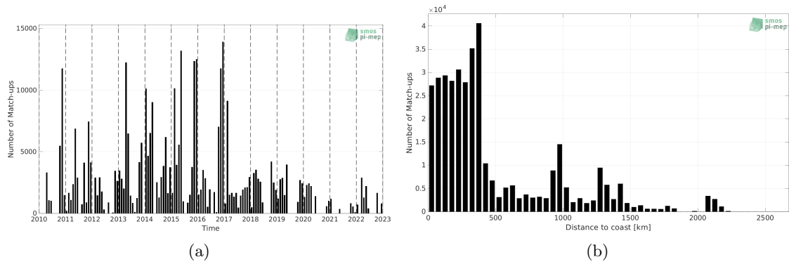
Figure 1: Number of match-ups between TSG (SAMOS) and SMOS SSS L2Q v331 - 0.25 Deg (CATDS-CPDC) SSS as a function of time (a) and as function of the distance to coast (b) over the Roaring Forties and Furious Fifties Pi-MEP region and for the full satellite product period.
