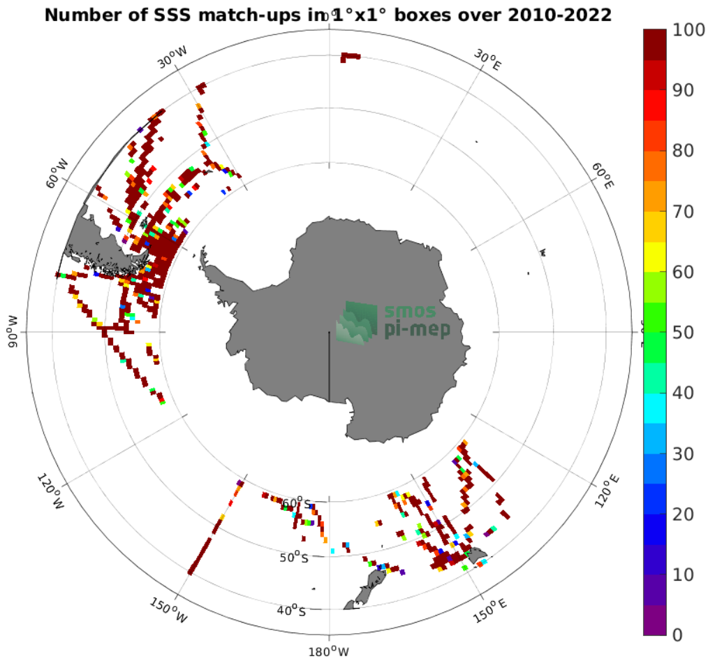
Figure 4: Number of SSS match-ups between TSG (SAMOS) SSS and the SMOS SSS L2Q v331 - 0.25 Deg (CATDS-CPDC) SSS product for the Roaring Forties and Furious Fifties Pi-MEP region over 1^\circ \times 1^\circ boxes and for the full satellite product period.
