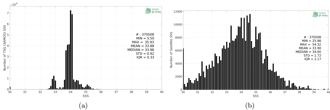
Figure 2: Histograms of SSS from TSG (SAMOS) (a) and SMOS SSS L2Q v331 - 0.25 Deg (CATDS-CPDC) (b) considering all match-up pairs per bins of 0.1 over the Roaring Forties and Furious Fifties Pi-MEP region and for the full satellite product period.
