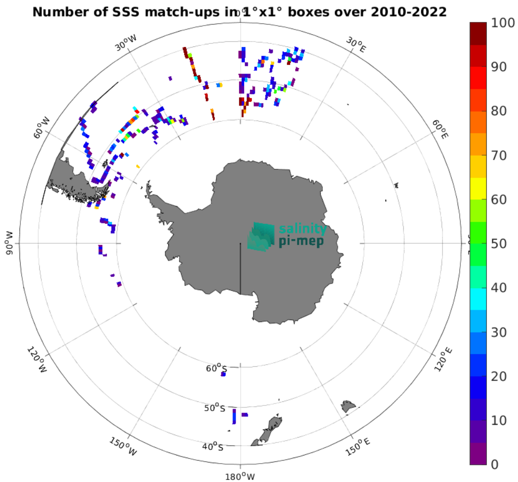
Figure 4: Number of SSS match-ups between TSG (Polarstern) SSS and the SMOS SSS L2Q v331 - 0.25 Deg (CATDS-CPDC) SSS product for the Roaring Forties and Furious Fifties Pi-MEP region over 1^{\circ} \times 1^{\circ} boxes and for the full satellite product period.
