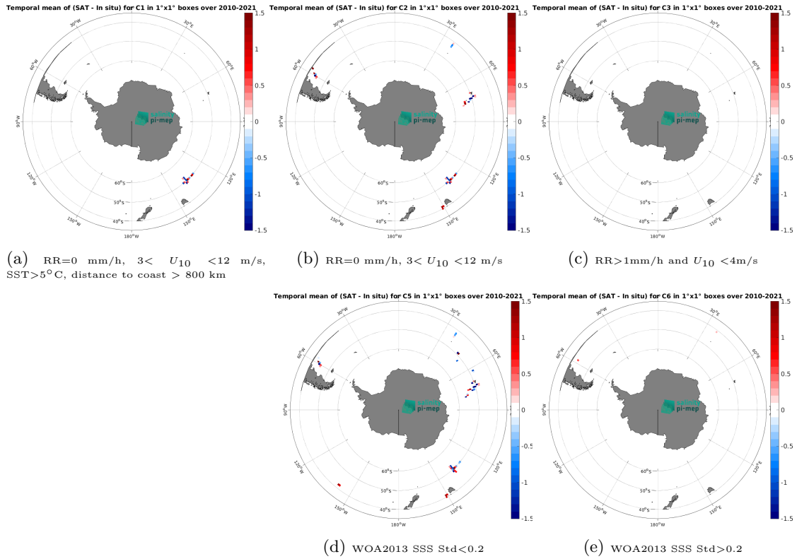
Figure 12: Temporal mean gridded over spatial boxes of size 1°×1° of \Delta SSS (SMOS SSS L2Q v331 - 0.25 Deg (CATDS-CPDC) - TSG (GOSUD-Research-vessel)) for 5 different subdatasets corresponding to:RR=0 mm/h, 3 < U_{10} < 12 m/s, SST>5°C, distance to coast > 800 km (a), RR=0 mm/h, 3 < U_{10} < 12 m/s (b), RR>1mm/h and U_{10} < 4 m/s (c), WOA2013 SSS Std<0.2 (d), WOA2013 SSS Std>0.2 (e).
