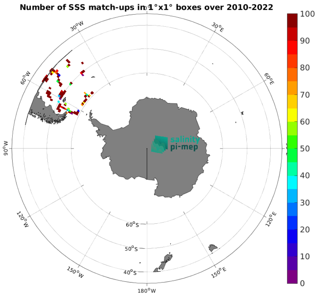
Figure 4: Number of SSS match-ups between TSG (CSIC-UTM) SSS and the SMOS SSS L2Q v331 - 0.25 Deg (CATDS-CPDC) SSS product for the Roaring Forties and Furious Fifties Pi-MEP region over 1^{\circ} \times 1^{\circ} boxes and for the full satellite product period.
