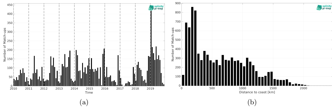
Figure 1: Number of match-ups between Marine mammals and SMOS SSS L2Q v331 - 0.25 Deg (CATDS-CPDC) SSS as a function of time (a) and as function of the distance to coast (b) over the Roaring Forties and Furious Fifties Pi-MEP region and for the full satellite product period.
