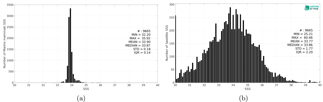
Figure 2: Histograms of SSS from Marine mammals (a) and SMOS SSS L2Q v331 - 0.25 Deg (CATDS-CPDC) (b) considering all match-up pairs per bins of 0.1 over the Roaring Forties and Furious Fifties Pi-MEP region and for the full satellite product period.
