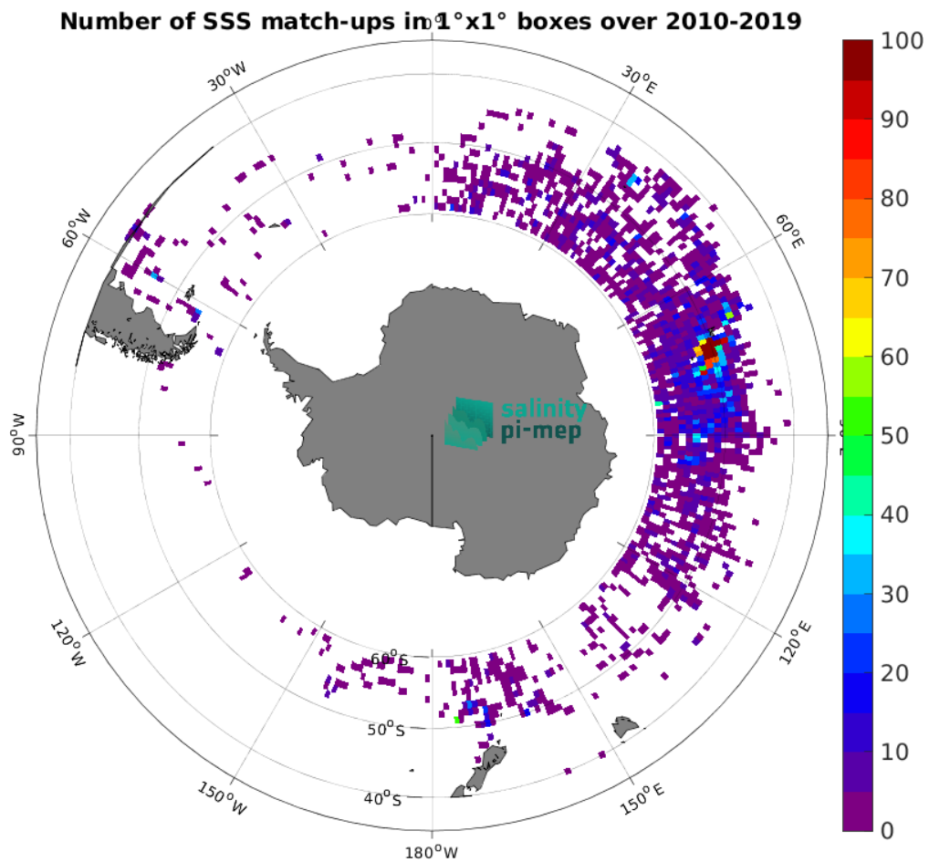
Figure 4: Number of SSS match-ups between Marine mammals SSS and the SMOS SSS L2Q v331 - 0.25 Deg (CATDS-CPDC) SSS product for the Roaring Forties and Furious Fifties Pi-MEP region over 1^\circ \times 1^\circ boxes and for the full satellite product period.
