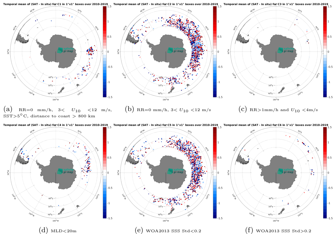
Figure 12: Temporal mean gridded over spatial boxes of size 1^{\circ}\times 1^{\circ} of \Delta\text{SSS} (SMOS SSS L2Q v331 - 0.25 Deg (CATDS-CPDC) - Marine mammals) for 6 different subdatasets corresponding to: RR=0 mm/h, 3 < U_{10} < 12 m/s, SST > 5^{\circ}\text{C} , distance to coast > 800 km (a), RR=0 mm/h, 3 < U_{10} < 12 m/s (b), RR > 1 mm/h and U_{10} < 4 m/s (c), MLD < 20 m (d), WOA2013 SSS Std < 0.2 (e), WOA2013 SSS Std > 0.2 (f).
