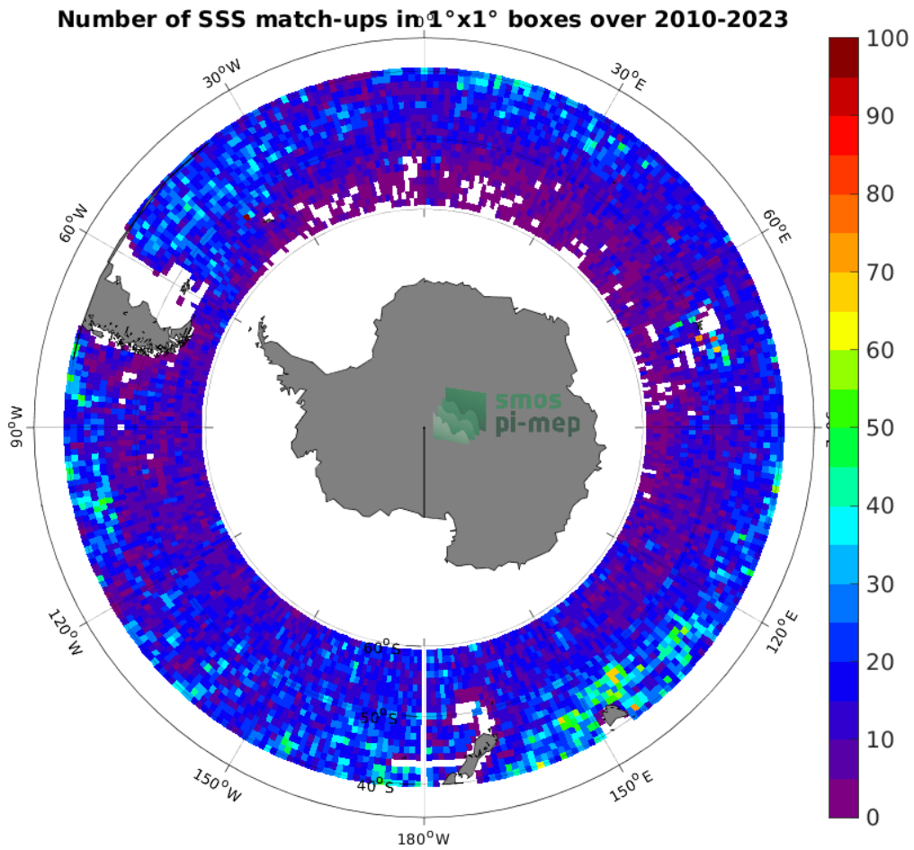
Figure 4: Number of SSS match-ups between Argo SSS and the SMOS SSS L2Q v331 - 0.25 Deg (CATDS-CPDC) SSS product for the Roaring Forties and Furious Fifties Pi-MEP region over 1^\circ \times 1^\circ boxes and for the full satellite product period.
