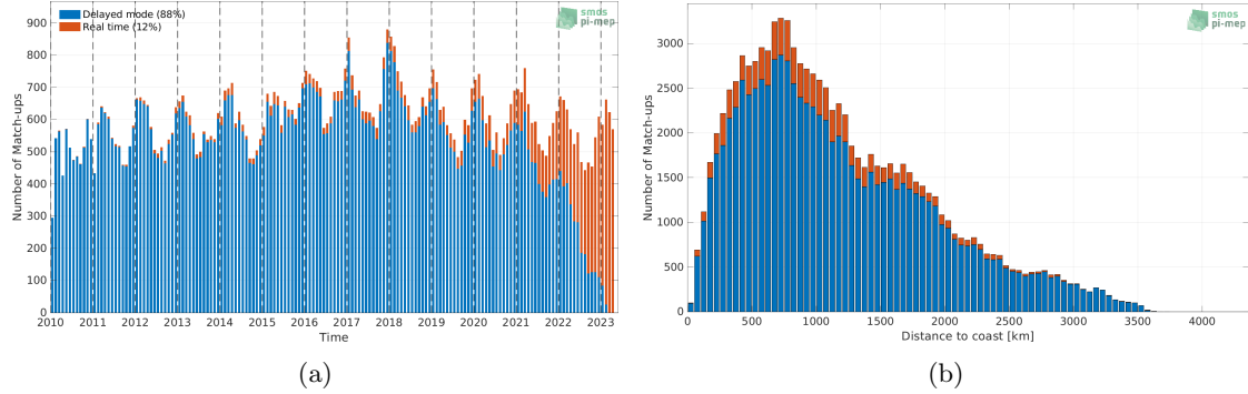
Figure 1: Number of match-ups between Argo and SMOS SSS L2Q v331 - 0.25 Deg (CATDS-CPDC) SSS as a function of time (a) and as function of the distance to coast (b) over the Roaring Forties and Furious Fifties Pi-MEP region and for the full satellite product period.
