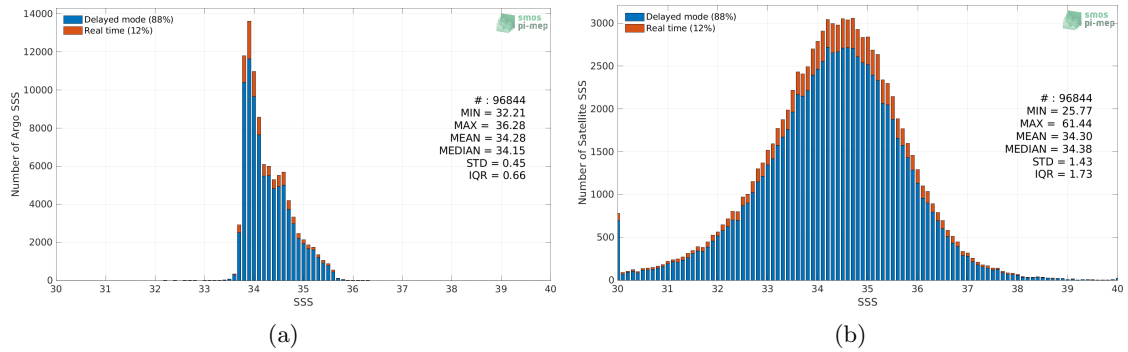
Figure 2: Histograms of SSS from Argo (a) and SMOS SSS L2Q v331 - 0.25 Deg (CATDS-CPDC) (b) considering all match-up pairs per bins of 0.1 over the Roaring Forties and Furious Fifties Pi-MEP region and for the full satellite product period.
