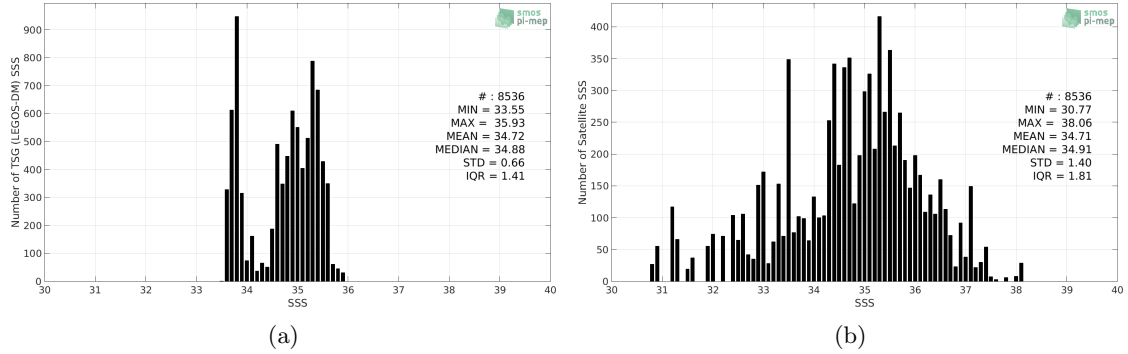
Figure 2: Histograms of SSS from TSG (LEGOS-DM) (a) and SMOS SSS L2Q v330 - 0.25 Deg (CATDS-CPDC) (b) considering all match-up pairs per bins of 0.1 over the Roaring Forties and Furious Fifties Pi-MEP region and for the full satellite product period.
