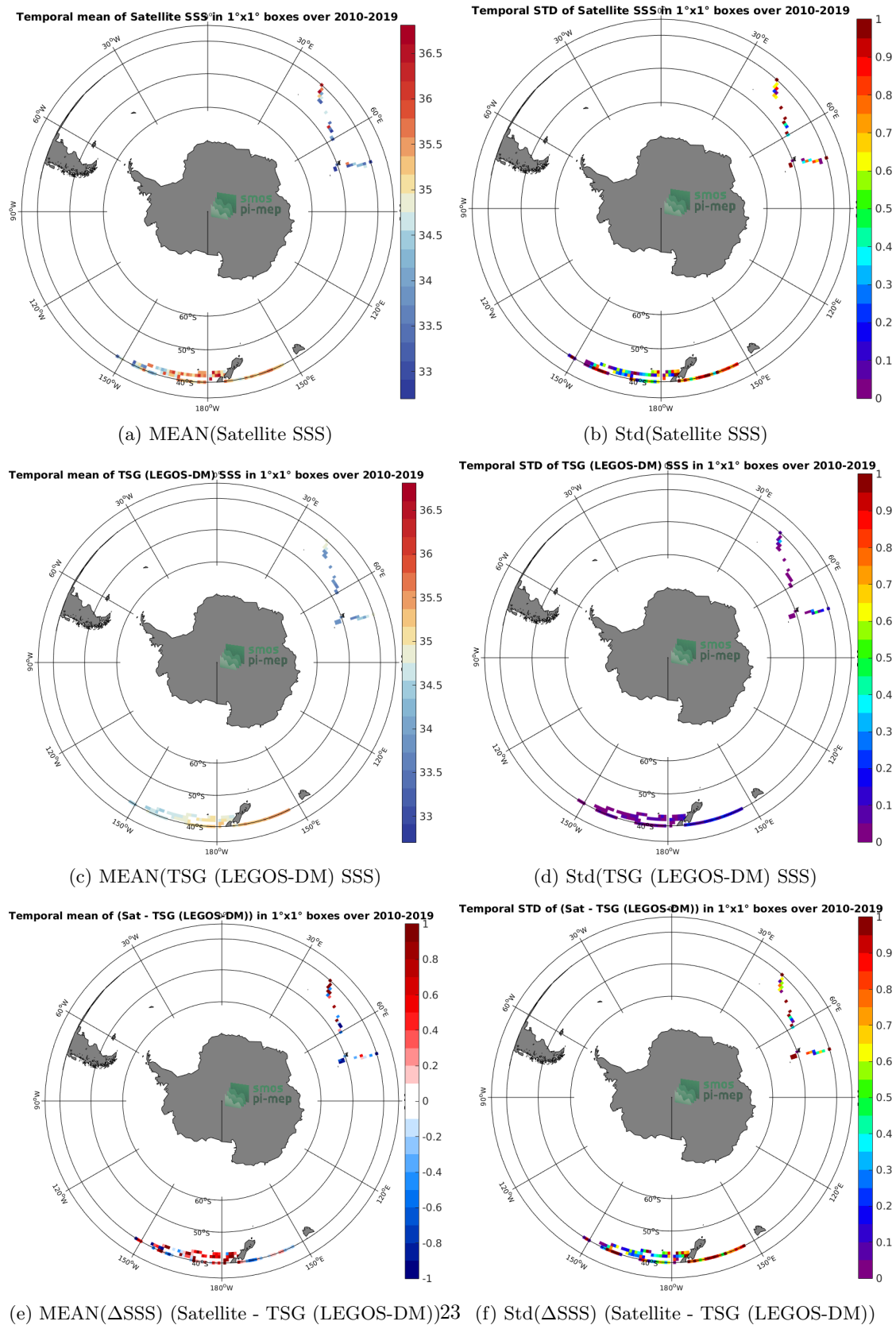
Figure 6: Temporal mean (left) and Std (right) of SSS from SMOS SSS L2Q v330 - 0.25 Deg (CATDS-CPDC) (top), TSG (LEGOS-DM) (middle), and of \Delta SSS (Satellite - TSG (LEGOS-DM)). Only match-up pairs are used to generate these maps.
