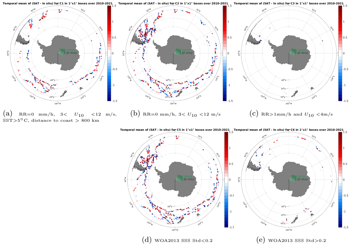
Figure 12: Temporal mean gridded over spatial boxes of size 1°×1° of \Delta SSS (SMOS SSS L2Q v330 - 0.25 Deg (CATDS-CPDC) - TSG (GOSUD-Sailing-ship)) for 5 different subdatasets corresponding to: RR=0 mm/h, 3 < U_{10} < 12 m/s, SST>5°C, distance to coast > 800 km (a), RR=0 mm/h, 3 < U_{10} < 12 m/s (b), RR>1mm/h and U_{10} < 4 m/s (c), WOA2013 SSS Std<0.2 (d), WOA2013 SSS Std>0.2 (e).
