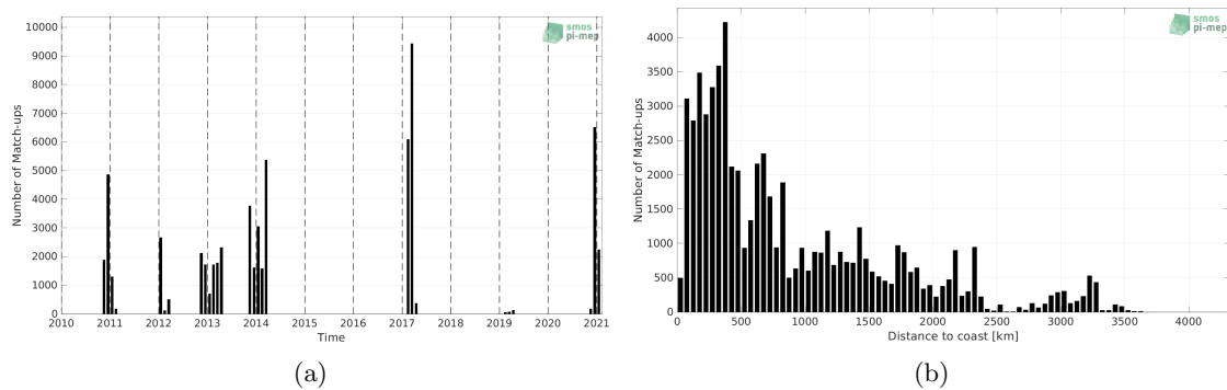
Figure 1: Number of match-ups between TSG (GOSUD-Sailing-ship) and SMOS SSS L2Q v330 - 0.25 Deg (CATDS-CPDC) SSS as a function of time (a) and as function of the distance to coast (b) over the Roaring Forties and Furious Fifties Pi-MEP region and for the full satellite product period.
