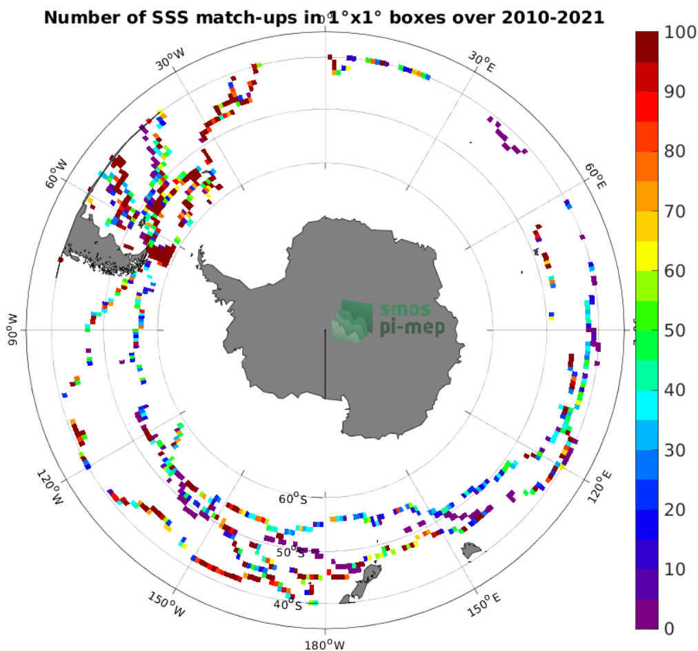
Figure 4: Number of SSS match-ups between TSG (GOSUD-Sailing-ship) SSS and the SMOS SSS L2Q v330 - 0.25 Deg (CATDS-CPDC) SSS product for the Roaring Forties and Furious Fifties Pi-MEP region over 1^\circ \times 1^\circ boxes and for the full satellite product period.
