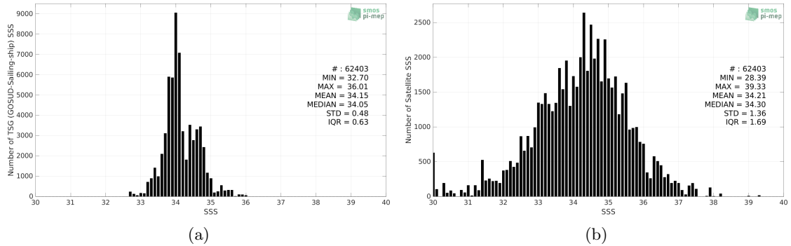
Figure 2: Histograms of SSS from TSG (GOSUD-Sailing-ship) (a) and SMOS SSS L2Q v330 - 0.25 Deg (CATDS-CPDC) (b) considering all match-up pairs per bins of 0.1 over the Roaring Forties and Furious Fifties Pi-MEP region and for the full satellite product period.
