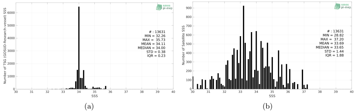
Figure 2: Histograms of SSS from TSG (GOSUD-Research-vessel) (a) and SMOS SSS L2Q v330 - 0.25 Deg (CATDS-CPDC) (b) considering all match-up pairs per bins of 0.1 over the Roaring Forties and Furious Fifties Pi-MEP region and for the full satellite product period.
