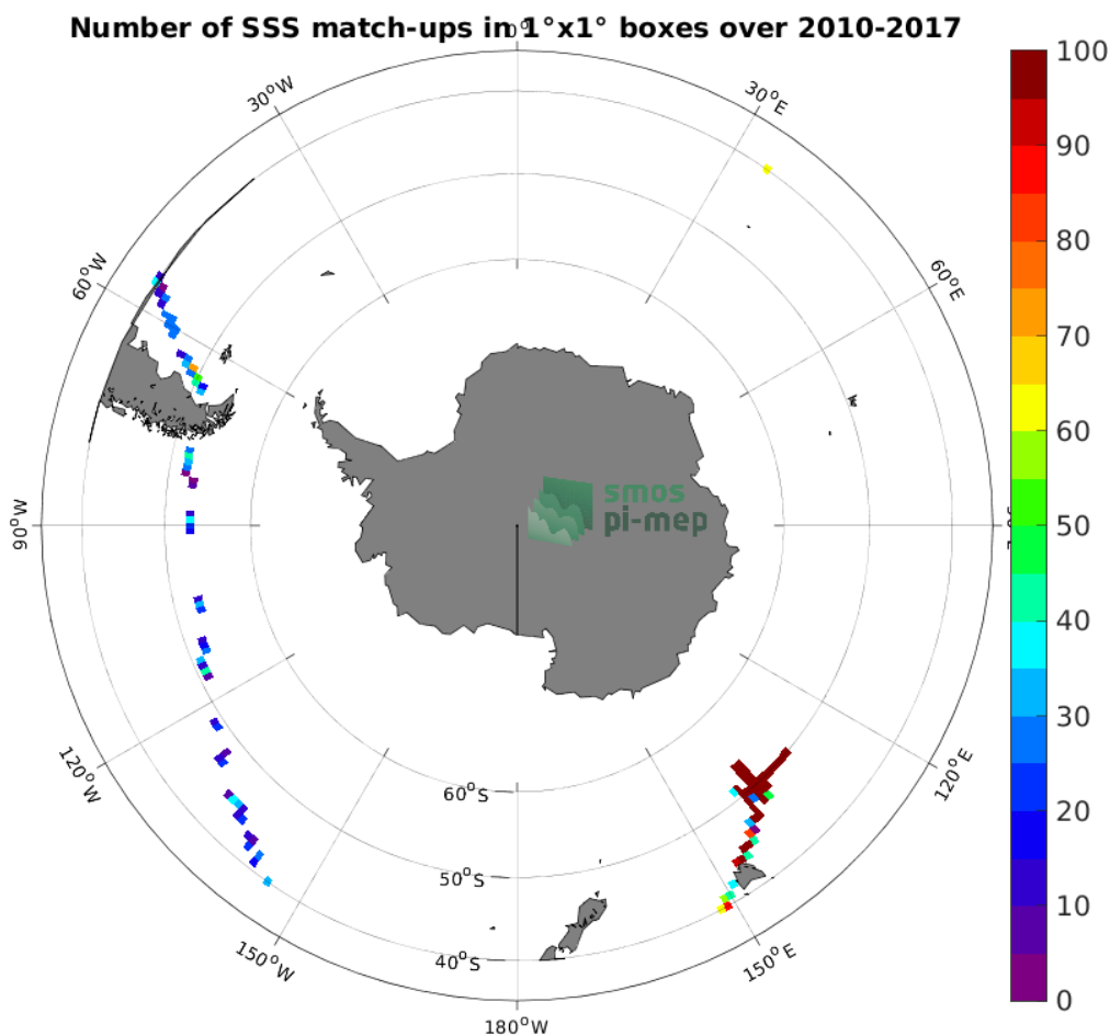
Figure 4: Number of SSS match-ups between TSG (GOSUD-Research-vessel) SSS and the SMOS SSS L2Q v330 - 0.25 Deg (CATDS-CPDC) SSS product for the Roaring Forties and Furious Fifties Pi-MEP region over 1^\circ \times 1^\circ boxes and for the full satellite product period.
