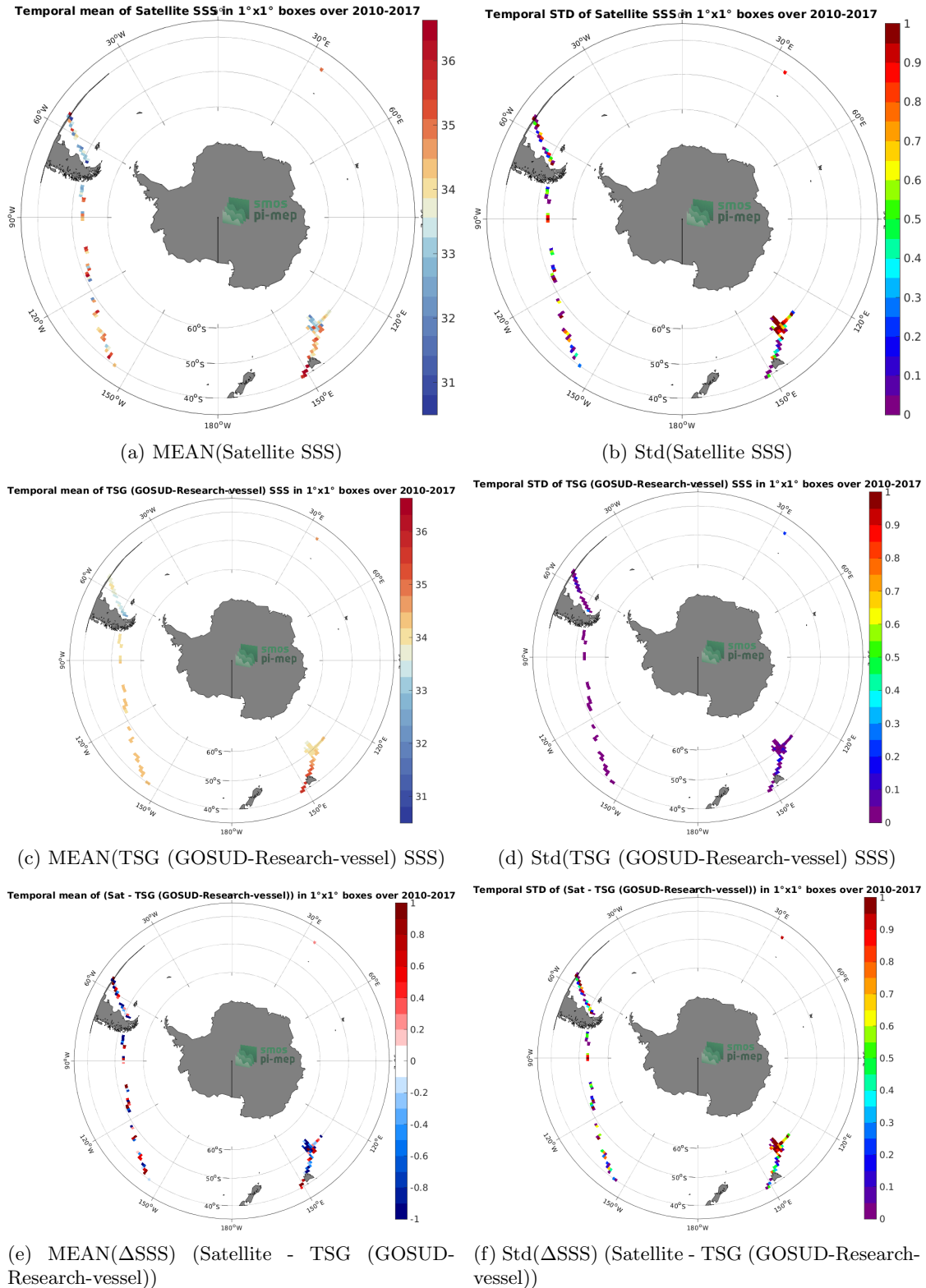
Figure 6: Temporal mean (left) and Std (right) of SSS from SMOS SSS L2Q v330 - 0.25 Deg (CATDS-CPDC) (top), TSG (GOSUD-Research-vessel) (middle), and of \Delta SSS (Satellite - TSG (GOSUD-Research-vessel)). Only match-up pairs are used to generate these maps.
