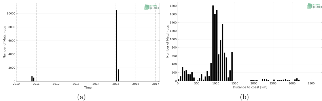
Figure 1: Number of match-ups between TSG (GOSUD-Research-vessel) and SMOS SSS L2Q v330 - 0.25 Deg (CATDS-CPDC) SSS as a function of time (a) and as function of the distance to coast (b) over the Roaring Forties and Furious Fifties Pi-MEP region and for the full satellite product period.
