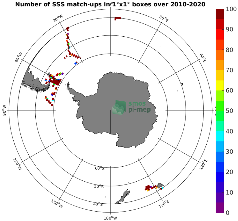
Figure 4: Number of SSS match-ups between TSG (SAMOS) SSS and the SMOS SSS L2Q v321 - 0.25 Deg (CATDS-CPDC) SSS product for the Roaring Forties and Furious Fifties Pi-MEP region over 1^\circ \times 1^\circ boxes and for the full satellite product period.
