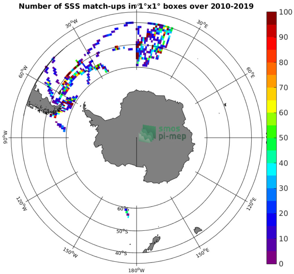
Figure 4: Number of SSS match-ups between TSG (Polarstern) SSS and the SMOS SSS L2Q v321 - 0.25 Deg (CATDS-CPDC) SSS product for the Roaring Forties and Furious Fifties Pi-MEP region over 1^\circ \times 1^\circ boxes and for the full satellite product period.
