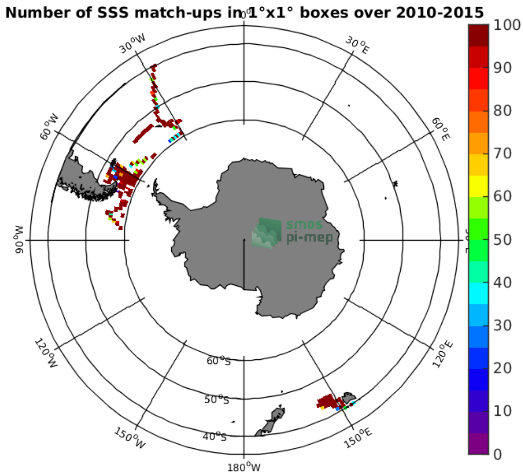
Figure 4: Number of SSS match-ups between TSG-SAMOS SSS and the SMOS-L3-CATDS-CPDC-V317-MONTHLY-25KM SSS product for the Roaring Forties and Furious Fifties Pi-MEP region over 1°x1° boxes and for the full satellite product period.
