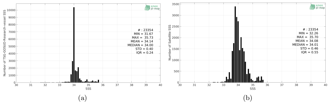
Figure 2: Histograms of SSS from TSG-GOSUD-Research-vessel (a) and SMOS L3 v317 - Monthly - 25 km (CATDS-CPDC) (b) considering all match-up pairs per bins of 0.1 over the Roaring Forties and Furious Fifties Pi-MEP region and for the full satellite product period.
