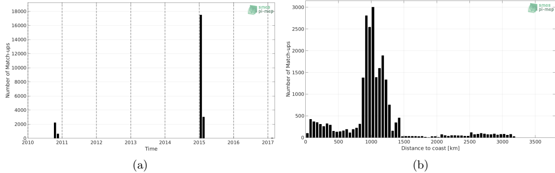
Figure 1: Number of match-ups between TSG-GOSUD-Research-vessel and SMOS L3 v317 - Monthly - 25 km (CATDS-CPDC) SSS as a function of time (a) and as function of the distance to coast (b) over the Roaring Forties and Furious Fifties Pi-MEP region and for the full satellite product period.
