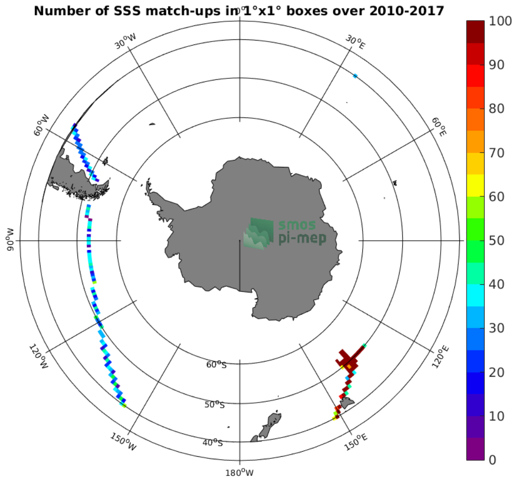
Figure 4: Number of SSS match-ups between TSG-GOSUD-Research-vessel SSS and the SMOS L3 v317 - Monthly - 25 km (CATDS-CPDC) SSS product for the Roaring Forties and Furious Fifties Pi-MEP region over 1°x1° boxes and for the full satellite product period.
