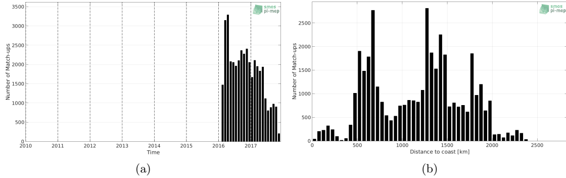
Figure 1: Number of match-ups between Surface drifters and SMOS-L3-CATDS-CPDC-V317-MONTHLY-25KM SSS as a function of time (a) and as function of the distance to coast (b) over the Roaring Forties and Furious Fifties Pi-MEP region and for the full satellite product period.
