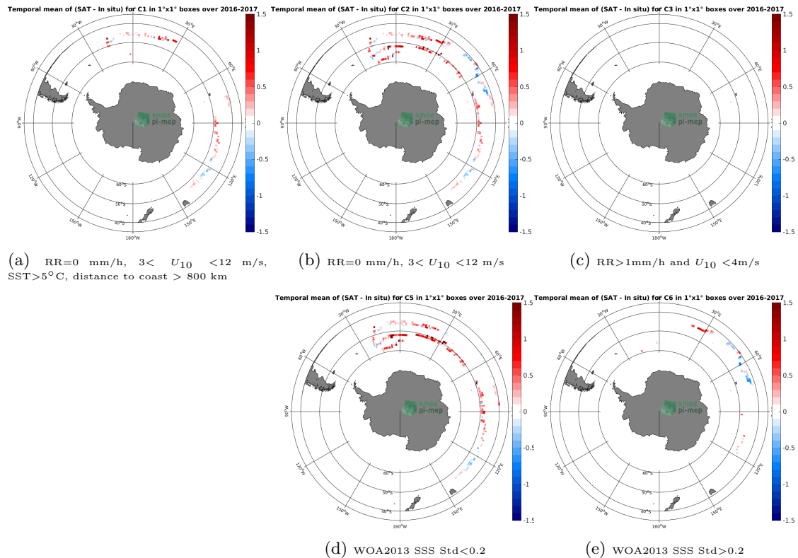
Figure 11: Temporal mean gridded over spatial boxes of size 1^\circ \times 1^\circ of \Delta SSS (SMOS-L3-CATDS-CPDC-V317-MONTHLY-25KM - Surface drifters) for 5 different subdatasets corresponding to:RR=0 mm/h, 3 < U_{10} < 12 m/s, SST >5^\circ C, distance to coast > 800 km (a), RR=0 mm/h, 3 < U_{10} < 12 m/s (b), RR >1 mm/h and U_{10} < 4 m/s (c), WOA2013 SSS Std <0.2 (d), WOA2013 SSS Std >0.2 (e).
