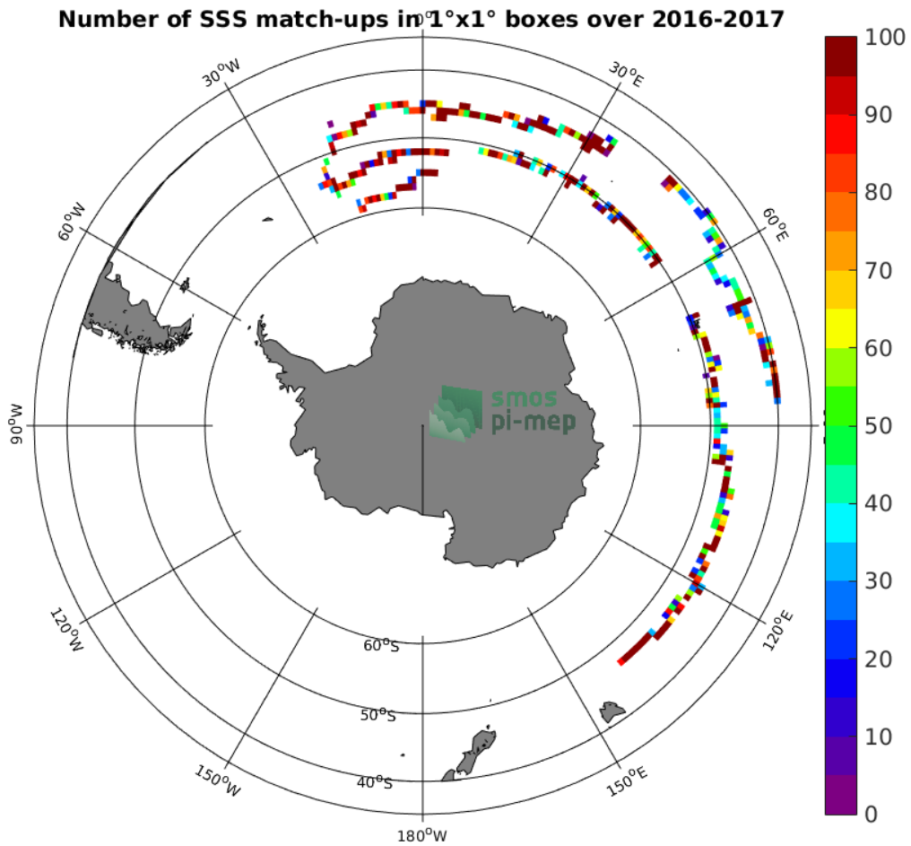
Figure 3: Number of SSS match-ups between Surface drifters SSS and the SMOS-L3-CATDS-CPDC-V317-MONTHLY-25KM SSS product for the Roaring Forties and Furious Fifties Pi-MEP region over 1^\circ \times 1^\circ boxes and for the full satellite product period.
