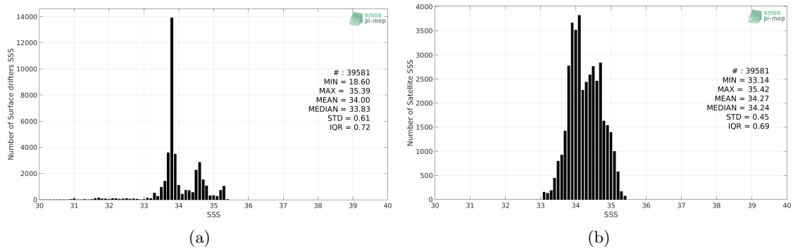
Figure 2: Histograms of SSS from Surface drifters (a) and SMOS-L3-CATDS-CPDC-V317-MONTHLY-25KM (b) considering all match-up pairs per bins of 0.1 over the Roaring Forties and Furious Fifties Pi-MEP region and for the full satellite product period.
