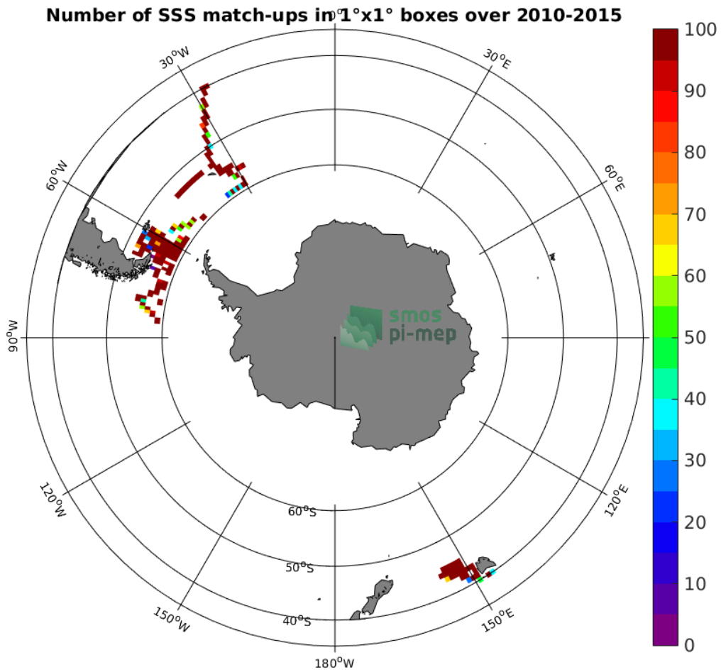
Figure 4: Number of SSS match-ups between TSG-SAMOS SSS and the SMOS-L3-CATDS-CPDC-V317-10DAYS-25KM SSS product for the Roaring Forties and Furious Fifties Pi-MEP region over 1°x1° boxes and for the full satellite product period.
