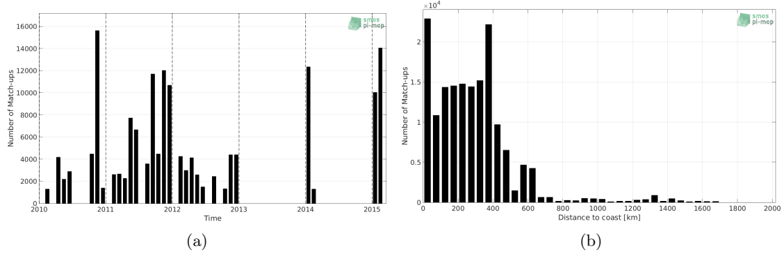
Figure 1: Number of match-ups between TSG-SAMOS and SMOS-L3-CATDS-CPDC-V317-10DAYS-25KM SSS as a function of time (a) and as function of the distance to coast (b) over the Roaring Forties and Furious Fifties Pi-MEP region and for the full satellite product period.
