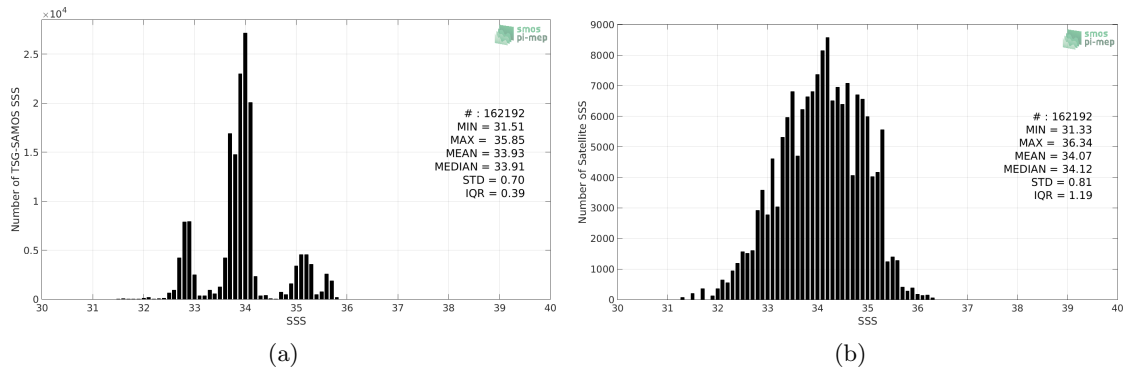
Figure 2: Histograms of SSS from TSG-SAMOS (a) and SMOS-L3-CATDS-CPDC-V317-10DAYS-25KM (b) considering all match-up pairs per bins of 0.1 over the Roaring Forties and Furious Fifties Pi-MEP region and for the full satellite product period.
