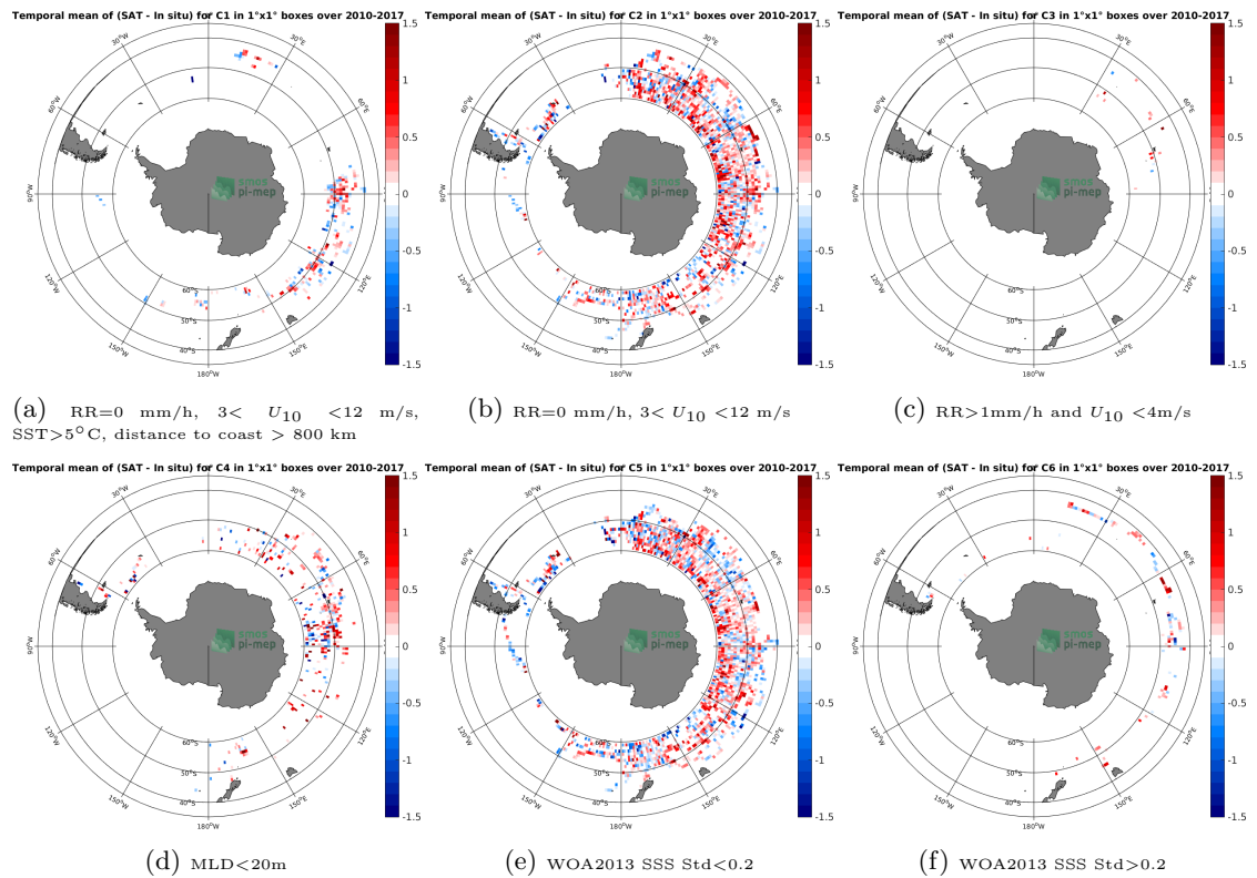
Figure 12: Temporal mean gridded over spatial boxes of size 1^\circ \times 1^\circ of \Delta SSS (SMOS-L3-CATDS-CPDC-V317-10DAYS-25KM - Sea mammals) for 6 different subdatasets corresponding to:RR=0 mm/h, 3 < U_{10} < 12 m/s, SST >5^\circ C, distance to coast > 800 km (a), RR=0 mm/h, 3 < U_{10} < 12 m/s (b), RR >1 mm/h and U_{10} < 4 m/s (c),MLD <20 m (d),WOA2013 SSS Std <0.2 (e),WOA2013 SSS Std >0.2 (f).
