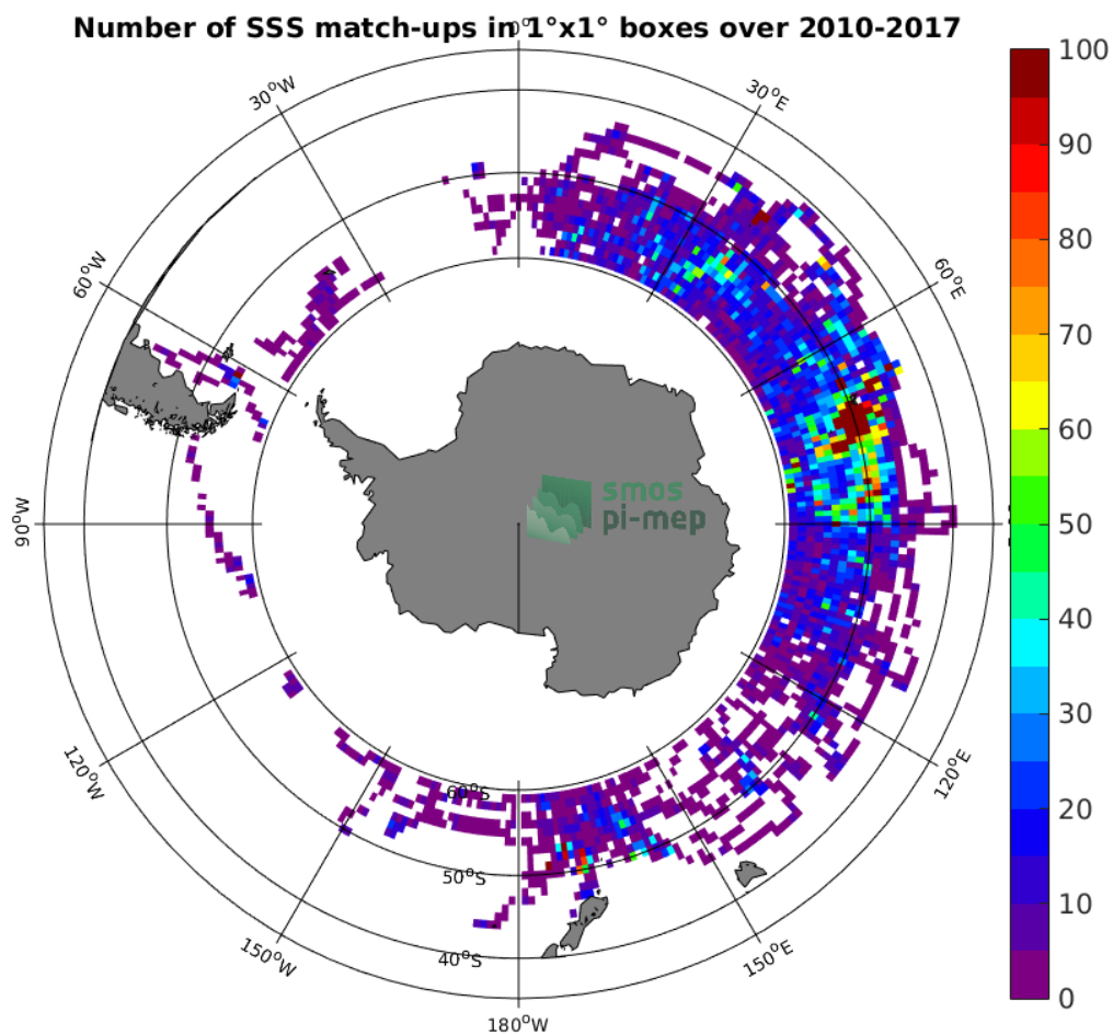
Figure 4: Number of SSS match-ups between Sea mammals SSS and the SMOS-L3-CATDS-CPDC-V317-10DAYS-25KM SSS product for the Roaring Forties and Furious Fifties Pi-MEP region over 1^\circ \times 1^\circ boxes and for the full satellite product period.
