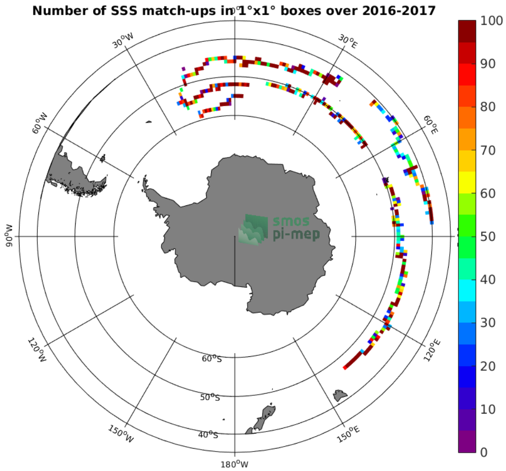
Figure 3: Number of SSS match-ups between Surface drifters SSS and the SMOS-L3-CATDS-CPDC-V317-10DAYS-25KM SSS product for the Roaring Forties and Furious Fifties Pi-MEP region over 1^\circ \times 1^\circ boxes and for the full satellite product period.
