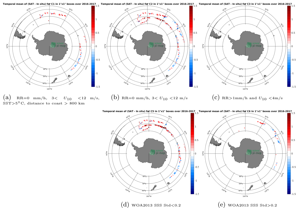
Figure 11: Temporal mean gridded over spatial boxes of size 1^\circ \times 1^\circ of \Delta SSS (SMOS-L3-CATDS-CPDC-V317-10DAYS-25KM - Surface drifters) for 5 different subdatasets corresponding to: RR=0 mm/h, 3 < U_{10} < 12 m/s, SST > 5^\circ\text{C} , distance to coast > 800 km (a), RR=0 mm/h, 3 < U_{10} < 12 m/s (b), RR > 1 mm/h and U_{10} < 4 m/s (c), WOA2013 SSS Std < 0.2 (d), WOA2013 SSS Std > 0.2 (e).
