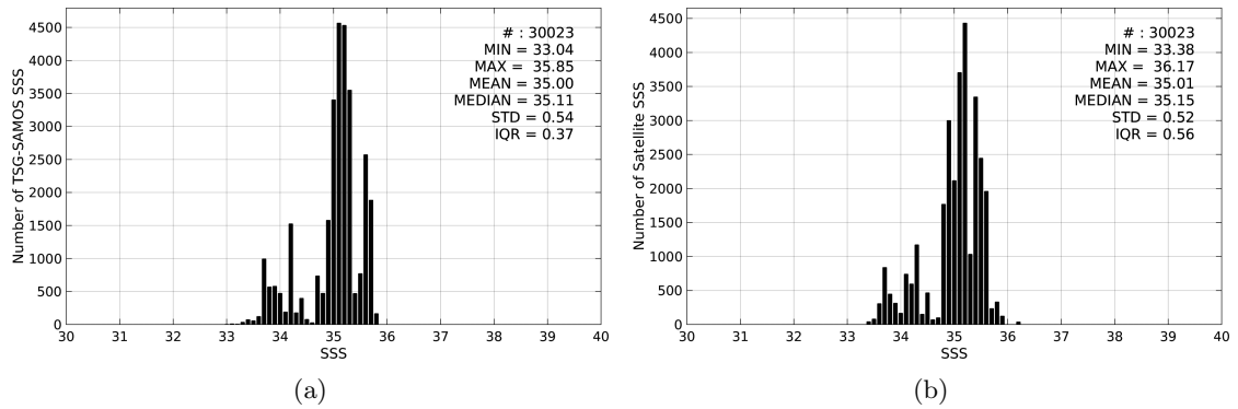
Figure 2: Histograms of SSS from TSG-SAMOS (a) and SMOS-L3-CATDS-CPDC-V3-MONTHLY-25KM (b) considering all match-up pairs per bins of 0.1 over the Roaring Forties and Furious Fifties Pi-MEP region and for the full satellite product period.
