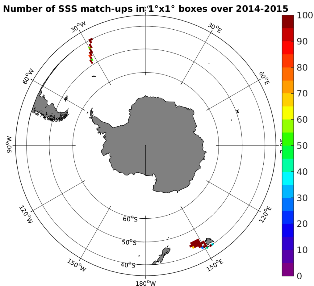
Figure 4: Number of SSS match-ups between TSG-SAMOS SSS and the SMOS-L3-CATDS-CPDC-V3-MONTHLY-25KM SSS product for the Roaring Forties and Furious Fifties Pi-MEP region over 1^\circ \times 1^\circ boxes and for the full satellite product period.
