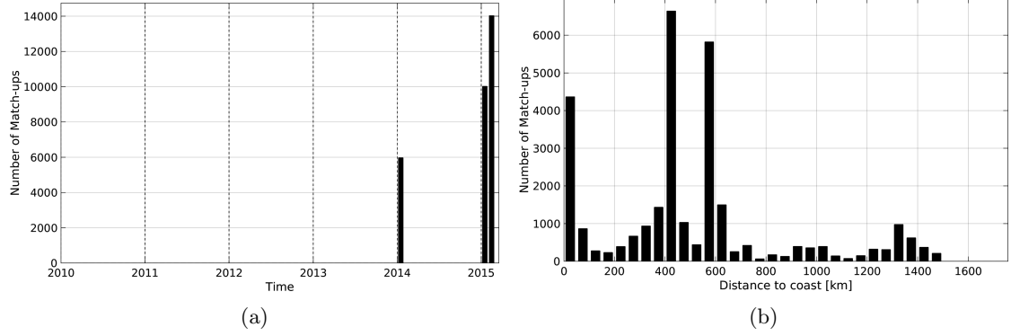
Figure 1: Number of match-ups between TSG-SAMOS and SMOS-L3-CATDS-CPDC-V3-MONTHLY-25KM SSS as a function of time (a) and as function of the distance to coast (b) over the Roaring Forties and Furious Fifties Pi-MEP region and for the full satellite product period.
