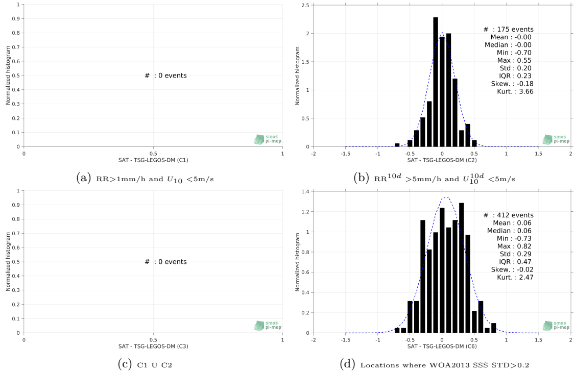
Figure 13: Normalized histogram of \Delta\text{SSS} (SMOS-L3-CATDS-CPDC-V3-MONTHLY-25KM - TSG-LEGOS-DM) for 6 different subdatasets corresponding to: RR > 1\text{mm/h} and U_{10} < 5\text{m/s} (a), RR^{10d} > 5\text{mm/h} and U_{10}^{10d} < 5\text{m/s} (b), C1 \cup C2 (c), Locations where WOA2013 SSS STD > 0.2 (d).
