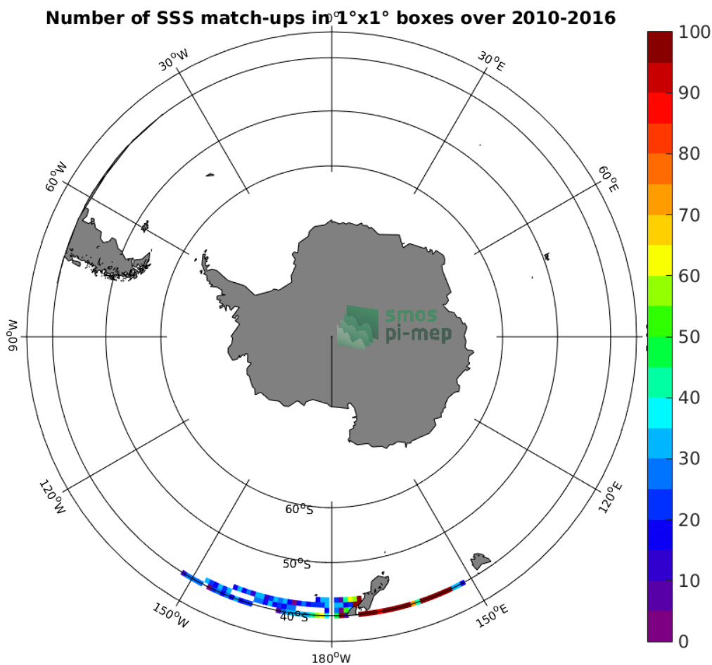
Figure 4: Number of SSS match-ups between TSG-LEGOS-DM SSS and the SMOS-L3-CATDS-CPDC-V3-MONTHLY-25KM SSS product for the Roaring Forties and Furious Fifties Pi-MEP region over 1°x1° boxes and for the full satellite product period.
