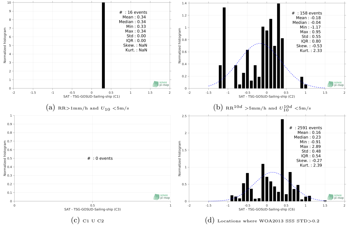
Figure 13: Normalized histogram of \Delta\text{SSS} (SMOS-L3-CATDS-CPDC-V3-MONTHLY-25KM - TSG-GOSUD-Sailing-ship) for 6 different subdatasets corresponding to: RR > 1mm/h and U_{10} < 5\text{m/s} (a), RR^{10d} > 5\text{mm/h} and U_{10}^{10d} < 5\text{m/s} (b), C1 U C2 (c), Locations where WOA2013 SSS STD > 0.2 (d).
