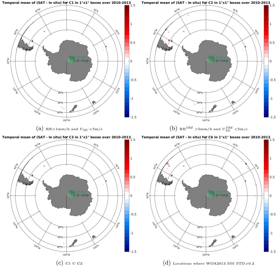
Figure 12: Temporal mean gridded over spatial boxes of size 1^\circ \times 1^\circ of \Delta SSS (SMOS-L3-CATDS-CPDC-V3-MONTHLY-25KM - TSG-GOSUD-Sailing-ship) for 4 different subdatasets corresponding to:RR >1 mm/h and U_{10} < 5 m/s (a), RR 10d > 5 mm/h and U_{10}^{10d} < 5 m/s (b), C1 U C2 (c),Locations where WOA2013 SSS STD >0.2 (d).
