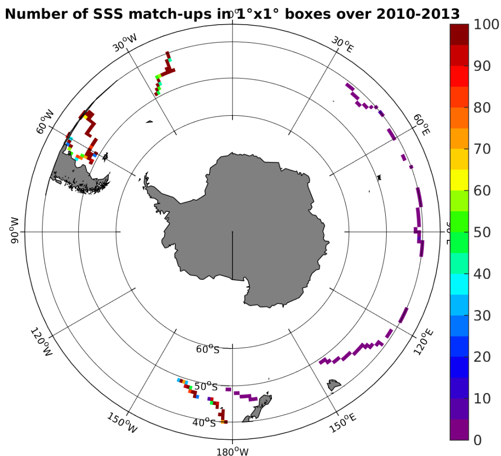
Figure 4: Number of SSS match-ups between TSG-GOSUD-Sailing-ship SSS and the SMOS-L3-CATDS-CPDC-V3-MONTHLY-25KM SSS product for the Roaring Forties and Furious Fifties Pi-MEP region over 1^\circ \times 1^\circ boxes and for the full satellite product period.
