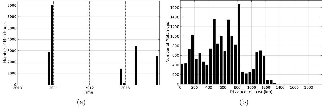
Figure 1: Number of match-ups between TSG-GOSUD-Sailing-ship and SMOS-L3-CATDS-CPDC-V3-MONTHLY-25KM SSS as a function of time (a) and as function of the distance to coast (b) over the Roaring Forties and Furious Fifties Pi-MEP region and for the full satellite product period.
