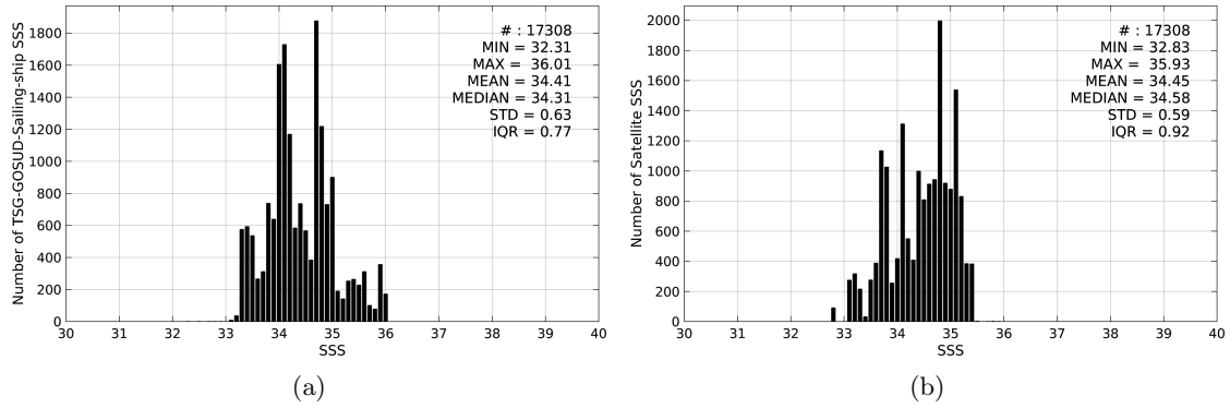
Figure 2: Histograms of SSS from TSG-GOSUD-Sailing-ship (a) and SMOS-L3-CATDS-CPDC-V3-MONTHLY-25KM (b) considering all match-up pairs per bins of 0.1 over the Roaring Forties and Furious Fifties Pi-MEP region and for the full satellite product period.
