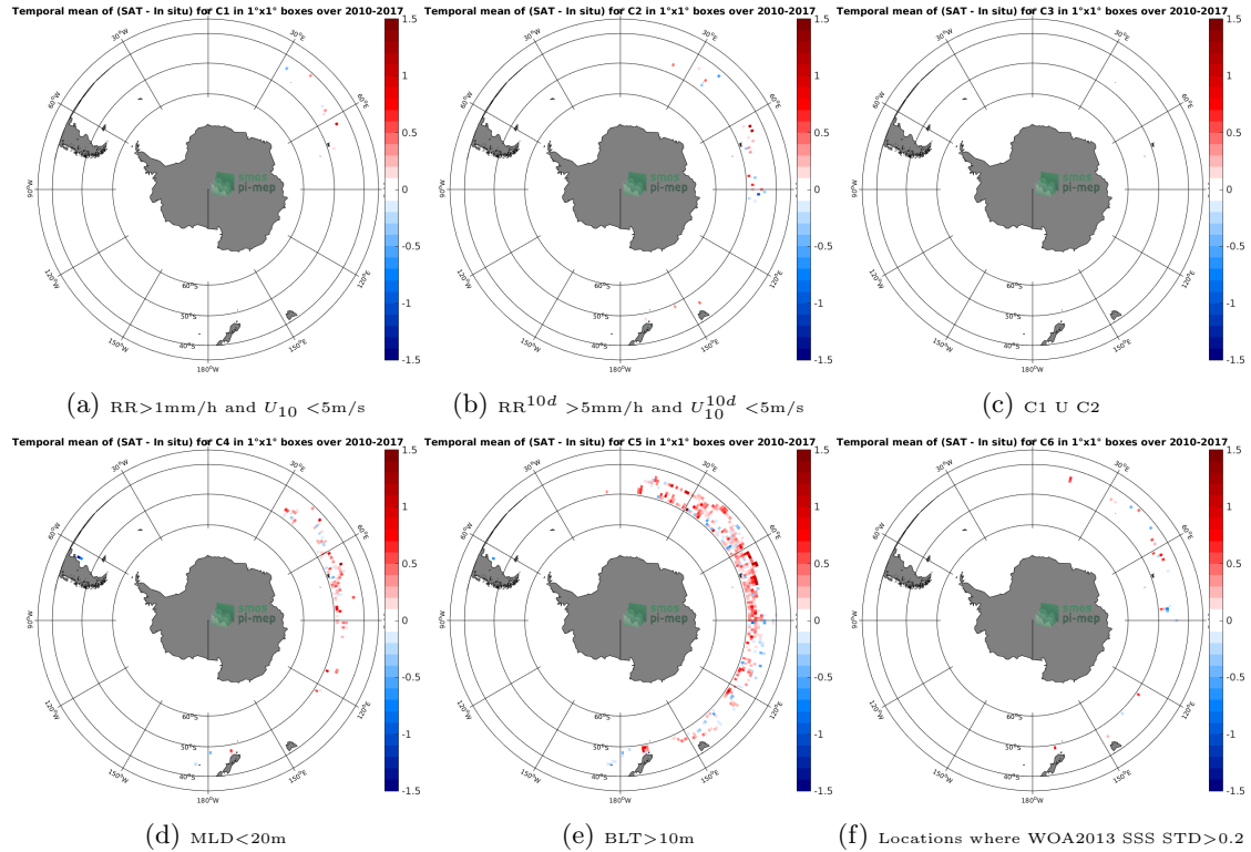
Figure 12: Temporal mean gridded over spatial boxes of size 1^\circ \times 1^\circ of \Delta SSS (SMOS-L3-CATDS-CPDC-V3-MONTHLY-25KM - Sea mammals) for 6 different subdatasets corresponding to: RR > 1\text{mm/h} and U_{10} < 5\text{m/s} (a), RR^{10d} > 5\text{mm/h} and U_{10}^{10d} < 5\text{m/s} (b), C1 U C2 (c), MLD < 20\text{m} (d), BLT > 10\text{m} (e), Locations where WOA2013 SSS STD > 0.2 (f).
