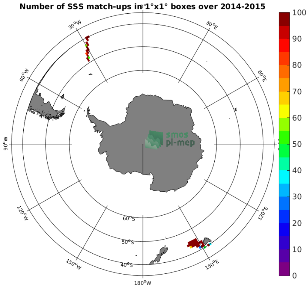
Figure 4: Number of SSS match-ups between TSG-SAMOS SSS and the SMOS-L3-CATDS-CPDC-V3-10DAYS-25KM SSS product for the Roaring Forties and Furious Fifties Pi-MEP region over 1°x1° boxes and for the full satellite product period.
