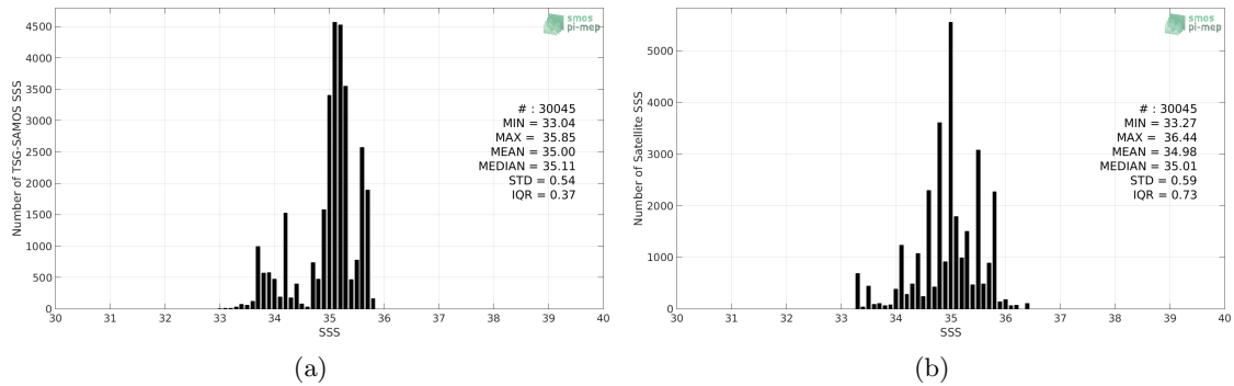
Figure 2: Histograms of SSS from TSG-SAMOS (a) and SMOS-L3-CATDS-CPDC-V3-10DAYS-25KM (b) considering all match-up pairs per bins of 0.1 over the Roaring Forties and Furious Fifties Pi-MEP region and for the full satellite product period.
