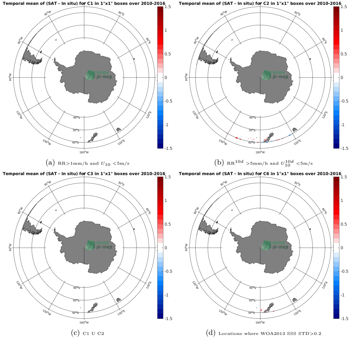
Figure 12: Temporal mean gridded over spatial boxes of size 1^\circ \times 1^\circ of \Delta SSS (SMOS-L3-CATDS-CPDC-V3-10DAYS-25KM - TSG-LEGOS-DM) for 4 different subdatasets corresponding to: RR > 1\text{mm/h} and U_{10} < 5\text{m/s} (a), RR^{10d} > 5\text{mm/h} and U_{10}^{10d} < 5\text{m/s} (b), C1 U C2 (c), Locations where WOA2013 SSS STD > 0.2 (d).
