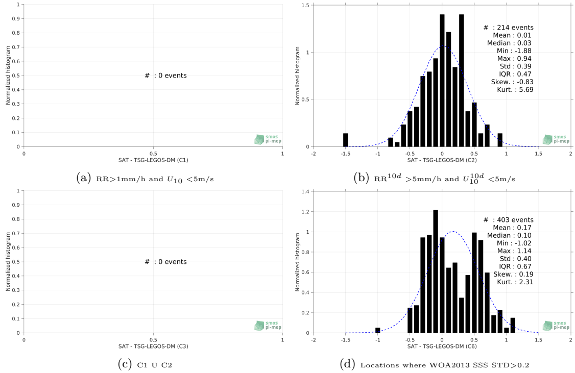
Figure 13: Normalized histogram of \Delta\text{SSS} (SMOS-L3-CATDS-CPDC-V3-10DAYS-25KM - TSG-LEGOS-DM) for 6 different subdatasets corresponding to: RR > 1\text{mm/h} and U_{10} < 5\text{m/s} (a), RR^{10d} > 5\text{mm/h} and U_{10}^{10d} < 5\text{m/s} (b), C1 \cup C2 (c), Locations where WOA2013 SSS STD > 0.2 (d).
