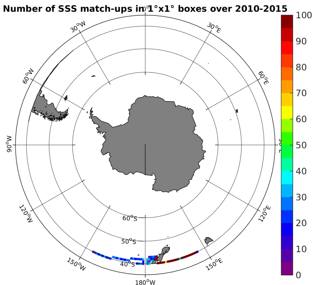
Figure 4: Number of SSS match-ups between TSG-LEGOS-DM SSS and the SMOS-L3-CATDS-CPDC-V3-10DAYS-25KM SSS product for the Roaring Forties and Furious Fifties Pi-MEP region over 1^\circ \times 1^\circ boxes and for the full satellite product period.
