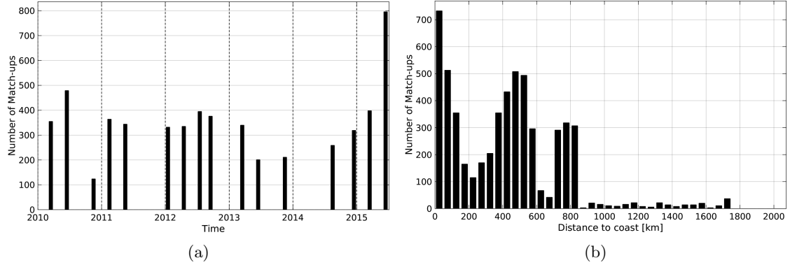
Figure 1: Number of match-ups between TSG-LEGOS-DM and SMOS-L3-CATDS-CPDC-V3-10DAYS-25KM SSS as a function of time (a) and as function of the distance to coast (b) over the Roaring Forties and Furious Fifties Pi-MEP region and for the full satellite product period.
