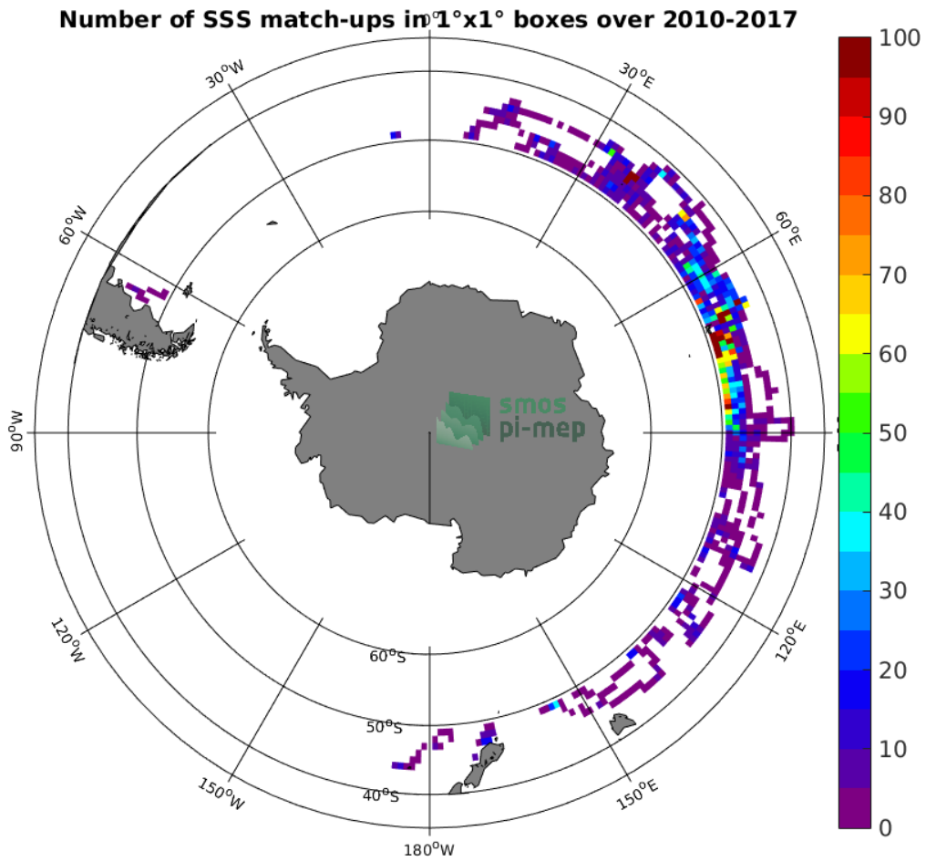
Figure 4: Number of SSS match-ups between Sea mammals SSS and the SMOS-L3-CATDS-CPDC-V3-10DAYS-25KM SSS product for the Roaring Forties and Furious Fifties Pi-MEP region over 1°x1° boxes and for the full satellite product period.
