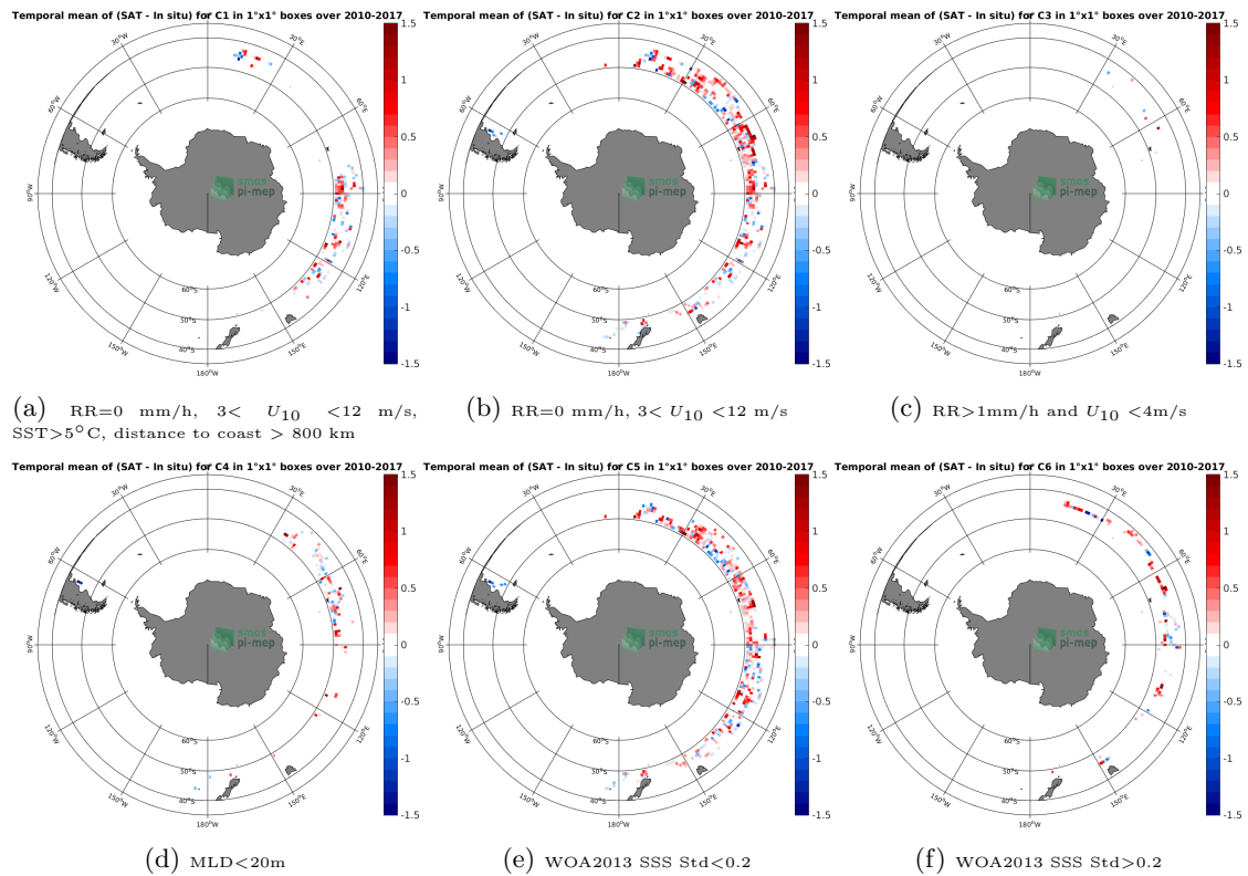
Figure 12: Temporal mean gridded over spatial boxes of size 1^\circ \times 1^\circ of \Delta SSS (SMOS-L3-CATDS-CPDC-V3-10DAYS-25KM - Sea mammals) for 6 different subdatasets corresponding to:RR=0 mm/h, 3 < U_{10} < 12 m/s, SST >5^\circ C, distance to coast > 800 km (a), RR=0 mm/h, 3 < U_{10} < 12 m/s (b), RR >1 mm/h and U_{10} < 4 m/s (c),MLD <20 m (d),WOA2013 SSS Std <0.2 (e),WOA2013 SSS Std >0.2 (f).
