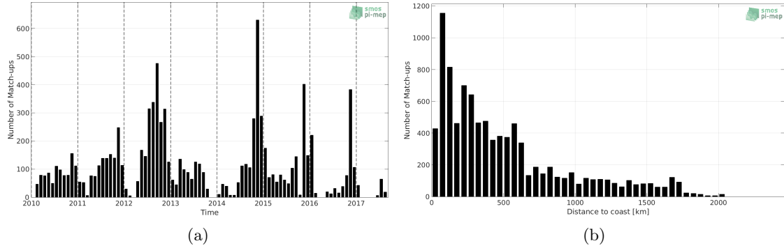
Figure 1: Number of match-ups between Sea mammals and SMOS-L3-CATDS-CPDC-V3-10DAYS-25KM SSS as a function of time (a) and as function of the distance to coast (b) over the Roaring Forties and Furious Fifties Pi-MEP region and for the full satellite product period.
