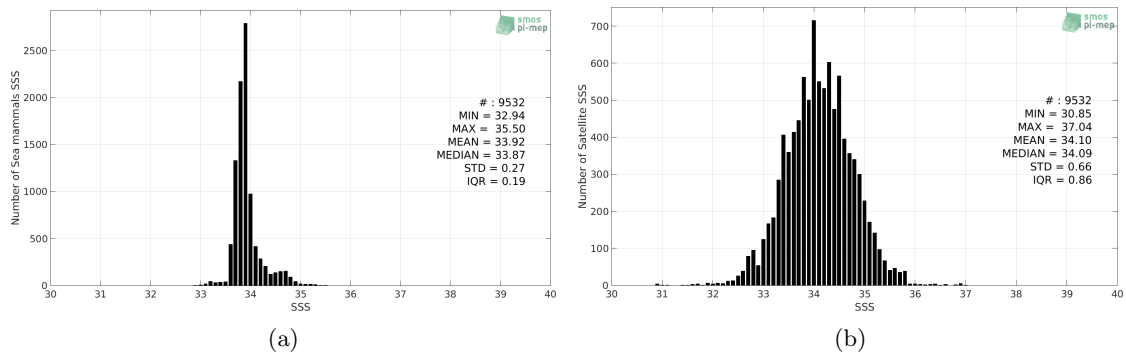
Figure 2: Histograms of SSS from Sea mammals (a) and SMOS-L3-CATDS-CPDC-V3-10DAYS-25KM (b) considering all match-up pairs per bins of 0.1 over the Roaring Forties and Furious Fifties Pi-MEP region and for the full satellite product period.
