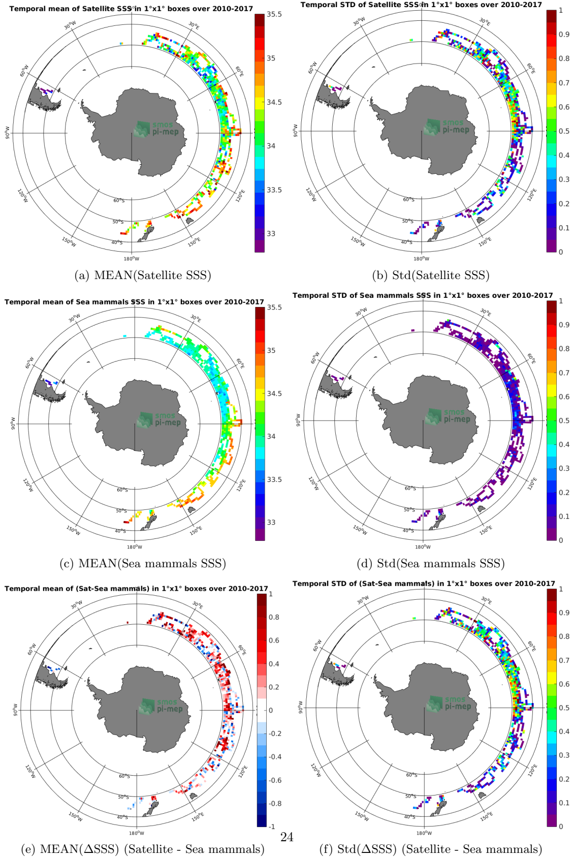
Figure 6: Temporal mean (left) and Std (right) of SSS from SMOS-L3-CATDS-CPDC-V3-10DAYS-25KM (top), Sea mammals (middle), and of \Delta SSS (Satellite - Sea mammals). Only match-up pairs are used to generate these maps.
