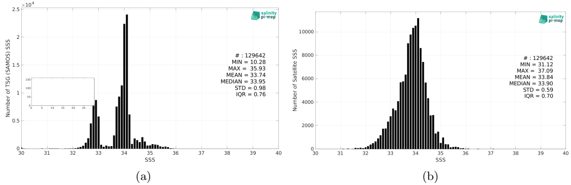
Figure 2: Histograms of SSS from TSG (SAMOS) (a) and SMOS SSS L3 v2 - 9-Days (BEC) (b) considering all match-up pairs per bins of 0.1 over the Roaring Forties and Furious Fifties Pi-MEP region and for the full satellite product period.
