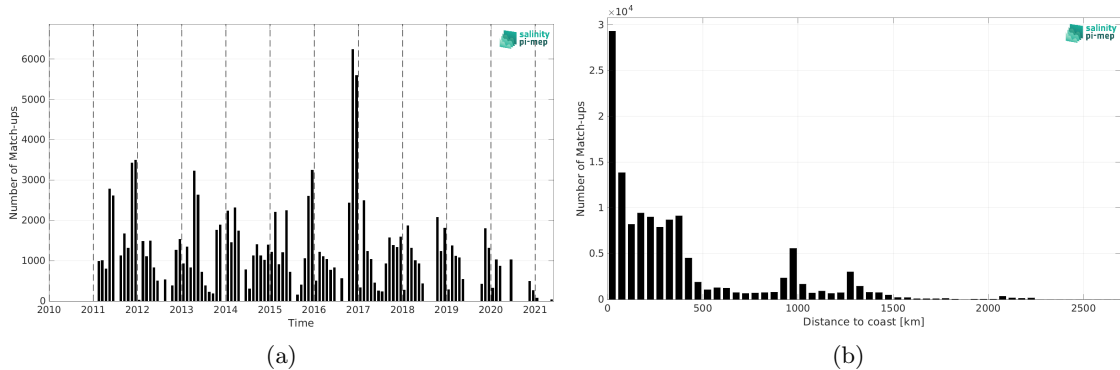
Figure 1: Number of match-ups between TSG (SAMOS) and SMOS SSS L3 v2 - 9-Days (BEC) SSS as a function of time (a) and as function of the distance to coast (b) over the Roaring Forties and Furious Fifties Pi-MEP region and for the full satellite product period.
