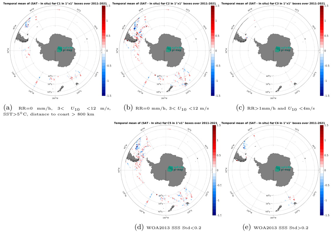
Figure 12: Temporal mean gridded over spatial boxes of size 1^{\circ}\times 1^{\circ} of \Delta\text{SSS} (SMOS SSS L3 v2 - 9-Days (BEC) - TSG (SAMOS)) for 5 different subdatasets corresponding to:RR=0 mm/h, 3 < U_{10} < 12 m/s, SST > 5^{\circ}\text{C} , distance to coast > 800 km (a), RR=0 mm/h, 3 < U_{10} < 12 m/s (b), RR > 1 mm/h and U_{10} < 4 m/s (c), WOA2013 SSS Std < 0.2 (d), WOA2013 SSS Std > 0.2 (e).
