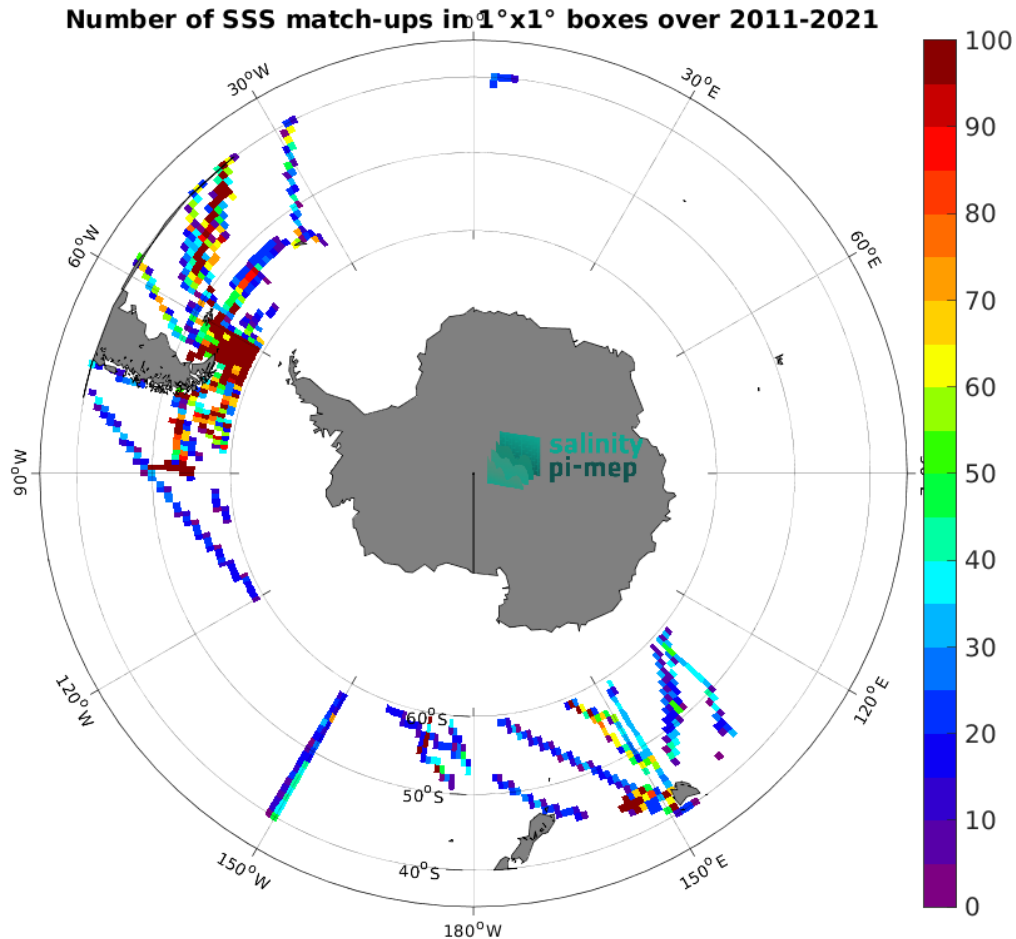
Figure 4: Number of SSS match-ups between TSG (SAMOS) SSS and the SMOS SSS L3 v2 - 9-Days (BEC) SSS product for the Roaring Forties and Furious Fifties Pi-MEP region over 1^\circ \times 1^\circ boxes and for the full satellite product period.
