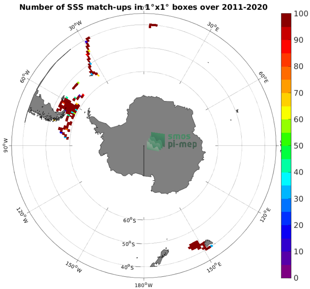
Figure 4: Number of SSS match-ups between TSG (SAMOS) SSS and the SMOS SSS L3 v2 - 9-Days (BEC) SSS product for the Roaring Forties and Furious Fifties Pi-MEP region over 1^\circ \times 1^\circ boxes and for the full satellite product period.
