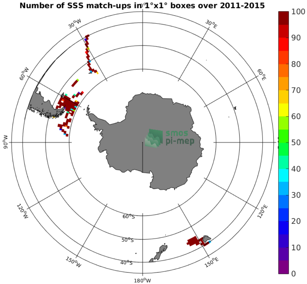
Figure 4: Number of SSS match-ups between TSG (SAMOS) SSS and the SMOS L3 v2 - 9-Days (BEC) SSS product for the Roaring Forties and Furious Fifties Pi-MEP region over 1°x1° boxes and for the full satellite product period.
