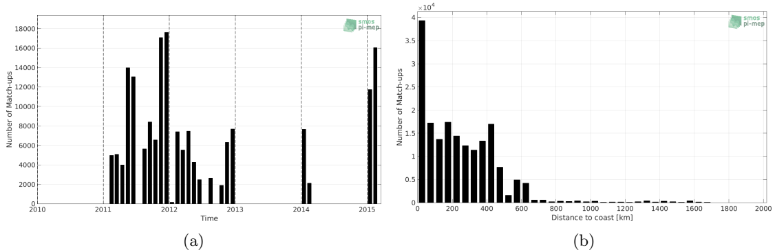
Figure 1: Number of match-ups between TSG (SAMOS) and SMOS L3 v2 - 9-Days (BEC) SSS as a function of time (a) and as function of the distance to coast (b) over the Roaring Forties and Furious Fifties Pi-MEP region and for the full satellite product period.
