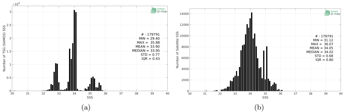
Figure 2: Histograms of SSS from TSG (SAMOS) (a) and SMOS L3 v2 - 9-Days (BEC) (b) considering all match-up pairs per bins of 0.1 over the Roaring Forties and Furious Fifties Pi-MEP region and for the full satellite product period.
