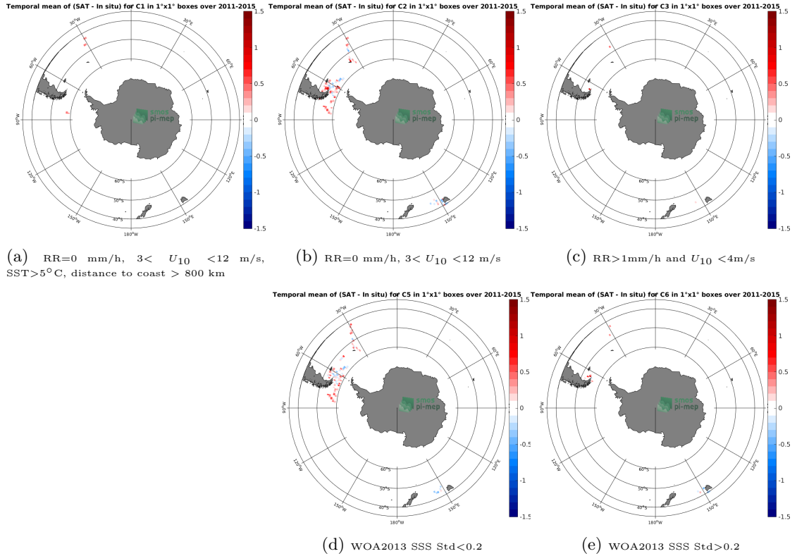
Figure 12: Temporal mean gridded over spatial boxes of size 1^{\circ}\times 1^{\circ} of \Delta\text{SSS} (SMOS L3 v2 - 9-Days (BEC) - TSG (SAMOS)) for 5 different subdatasets corresponding to:RR=0 mm/h, 3 < U_{10} < 12 m/s, SST >5^{\circ}\text{C} , distance to coast > 800 km (a), RR=0 mm/h, 3 < U_{10} < 12 m/s (b), RR >1 mm/h and U_{10} < 4 m/s (c), WOA2013 SSS Std <0.2 (d), WOA2013 SSS Std >0.2 (e).
