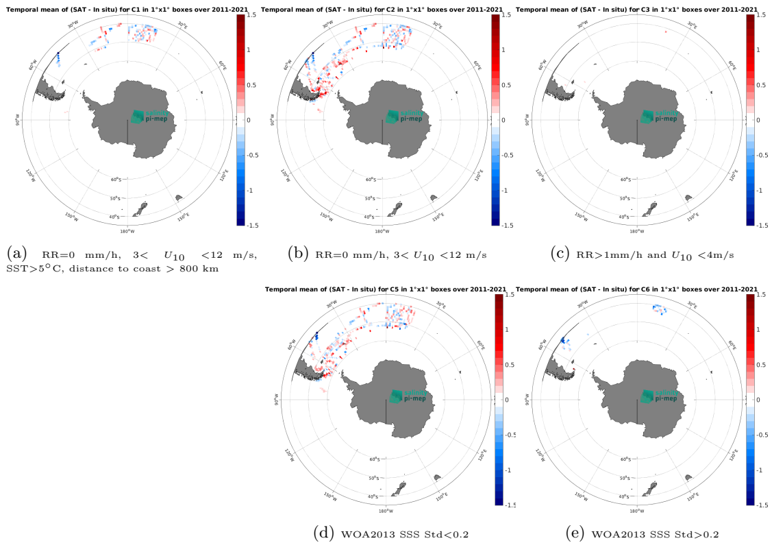
Figure 14: Temporal mean gridded over spatial boxes of size 1^\circ \times 1^\circ of \Delta SSS (SMOS SSS L3 v2 - 9-Days (BEC) - TSG (Polarstern)) for 5 different subdatasets corresponding to:RR=0 mm/h, 3 < U_{10} < 12 m/s, SST>5°C, distance to coast > 800 km (a), RR=0 mm/h, 3 < U_{10} < 12 m/s (b), RR>1mm/h and U_{10} < 4 m/s (c), WOA2013 SSS Std<0.2 (d), WOA2013 SSS Std>0.2 (e).
