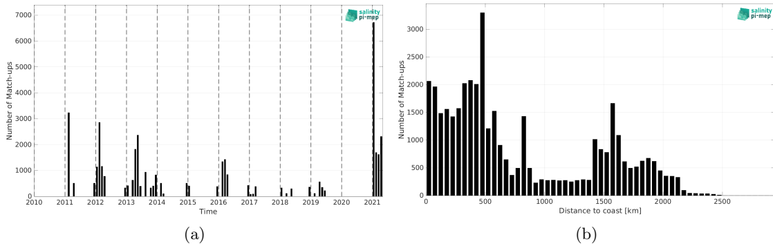
Figure 2: Number of match-ups between TSG (Polarstern) and SMOS SSS L3 v2 - 9-Days (BEC) SSS as a function of time (a) and as function of the distance to coast (b) over the Roaring Forties and Furious Fifties Pi-MEP region and for the full satellite product period.
