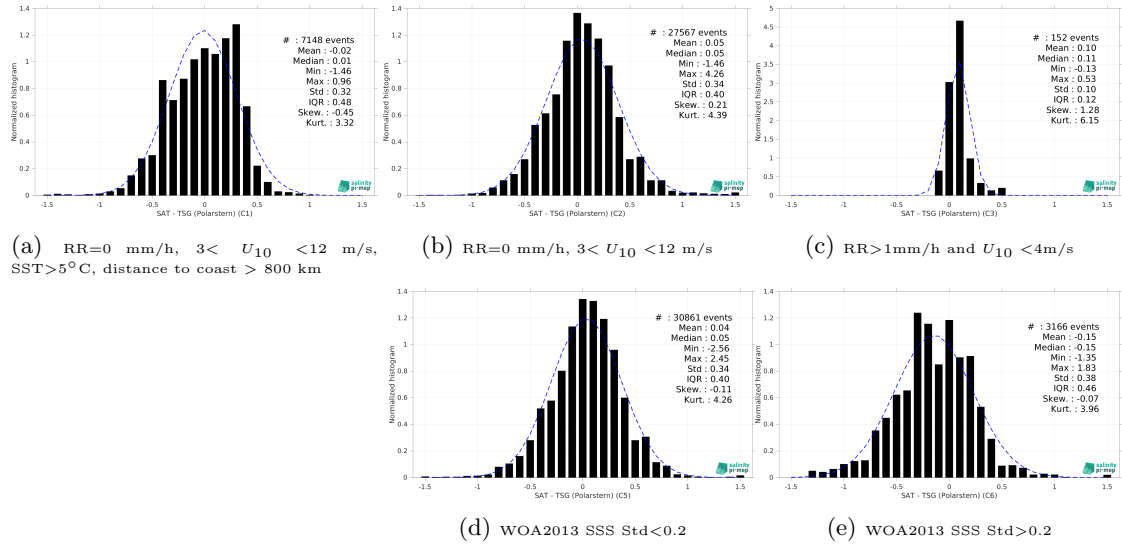
Figure 15: Normalized histogram of \Delta SSS (SMOS SSS L3 v2 - 9-Days (BEC) - TSG (Polarstern)) for 5 different subdatasets corresponding to: RR=0 mm/h, 3 < U_{10} < 12 m/s, SST > 5°C, distance to coast > 800 km (a), RR=0 mm/h, 3 < U_{10} < 12 m/s (b), RR > 1mm/h and U_{10} < 4 m/s (c), WOA2013 SSS Std < 0.2 (d), WOA2013 SSS Std > 0.2 (e).
