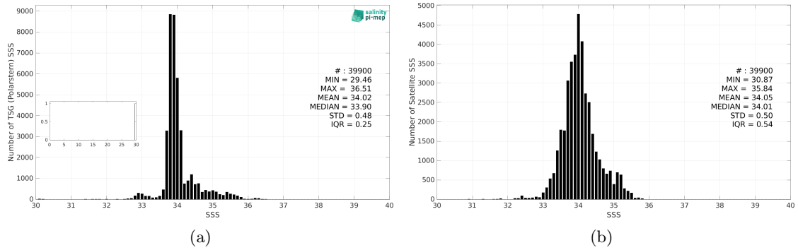
Figure 3: Histograms of SSS from TSG (Polarstern) (a) and SMOS SSS L3 v2 - 9-Days (BEC) (b) considering all match-up pairs per bins of 0.1 over the Roaring Forties and Furious Fifties Pi-MEP region and for the full satellite product period.
