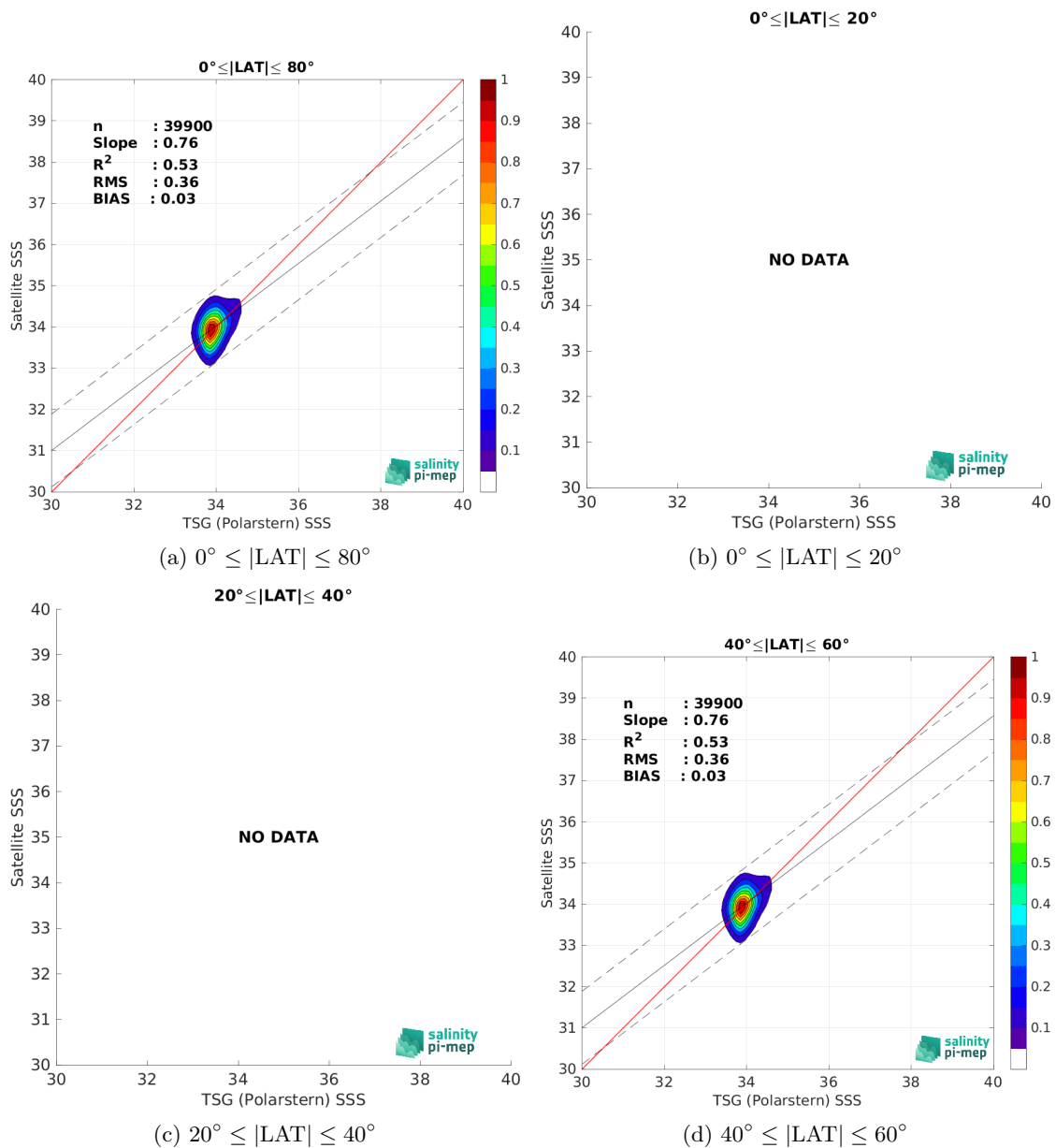
Figure 10: Contour maps of the concentration of SMOS SSS L3 v2 - 9-Days (BEC) SSS (y-axis) versus TSG (Polarstern) SSS (x-axis) at match-up pairs for different latitude bands. For each plot, the red line shows x=y . The black thin and dashed lines indicate a linear fit through the data cloud and the \pm 95\% confidence levels, respectively. The number match-up pairs n , the slope and R^2 coefficient of the linear fit, the root mean square (RMS) and the mean bias between satellite and in situ data are indicated for each latitude band in each plots.
