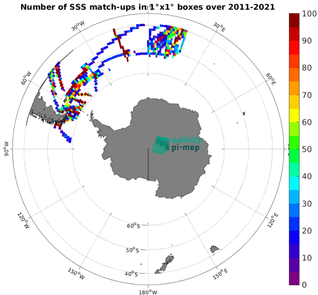
Figure 5: Number of SSS match-ups between TSG (Polarstern) SSS and the SMOS SSS L3 v2 - 9-Days (BEC) SSS product for the Roaring Forties and Furious Fifties Pi-MEP region over 1^\circ \times 1^\circ boxes and for the full satellite product period.
