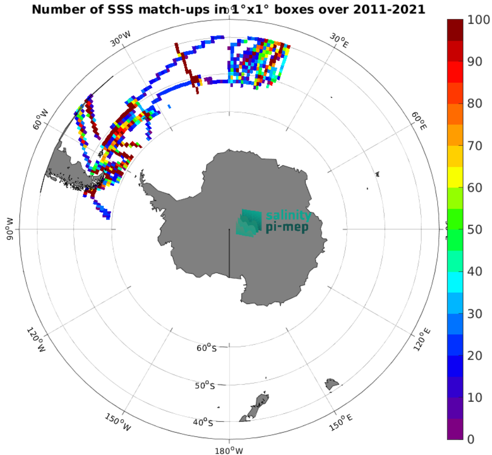
Figure 4: Number of SSS match-ups between TSG (Polarstern) SSS and the SMOS SSS L3 v2 - 9-Days (BEC) SSS product for the Roaring Forties and Furious Fifties Pi-MEP region over 1^\circ \times 1^\circ boxes and for the full satellite product period.
