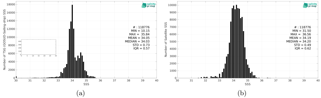
Figure 2: Histograms of SSS from TSG (GOSUD-Sailing-ship) (a) and SMOS SSS L3 v2 - 9-Days (BEC) (b) considering all match-up pairs per bins of 0.1 over the Roaring Forties and Furious Fifties Pi-MEP region and for the full satellite product period.
