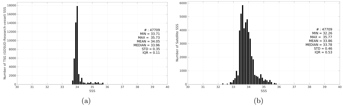
Figure 3: Histograms of SSS from TSG (GOSUD-Research-vessel) (a) and SMOS SSS L3 v2 - 9-Days (BEC) (b) considering all match-up pairs per bins of 0.1 over the Roaring Forties and Furious Fifties Pi-MEP region and for the full satellite product period.
