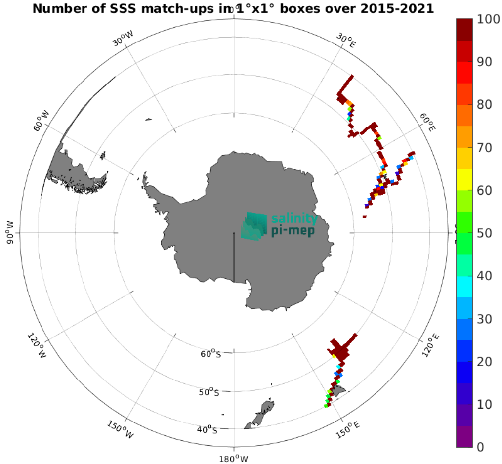
Figure 5: Number of SSS match-ups between TSG (GOSUD-Research-vessel) SSS and the SMOS SSS L3 v2 - 9-Days (BEC) SSS product for the Roaring Forties and Furious Fifties Pi-MEP region over 1^\circ \times 1^\circ boxes and for the full satellite product period.
