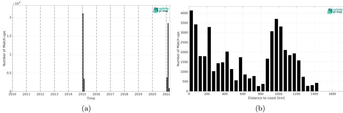
Figure 2: Number of match-ups between TSG (GOSUD-Research-vessel) and SMOS SSS L3 v2 - 9-Days (BEC) SSS as a function of time (a) and as function of the distance to coast (b) over the Roaring Forties and Furious Fifties Pi-MEP region and for the full satellite product period.
