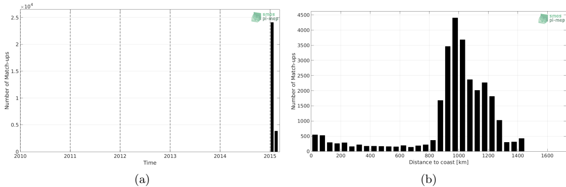
Figure 1: Number of match-ups between TSG (GOSUD-Research-vessel) and SMOS L3 v2 - 9-Days (BEC) SSS as a function of time (a) and as function of the distance to coast (b) over the Roaring Forties and Furious Fifties Pi-MEP region and for the full satellite product period.
