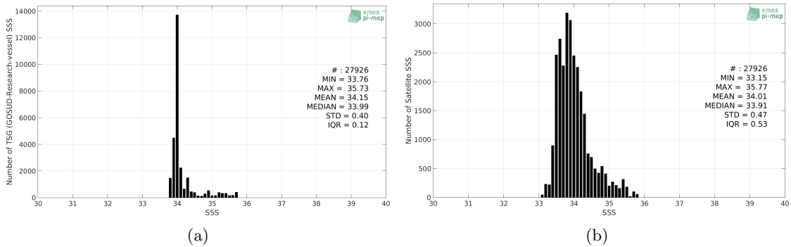
Figure 2: Histograms of SSS from TSG (GOSUD-Research-vessel) (a) and SMOS L3 v2 - 9-Days (BEC) (b) considering all match-up pairs per bins of 0.1 over the Roaring Forties and Furious Fifties Pi-MEP region and for the full satellite product period.
