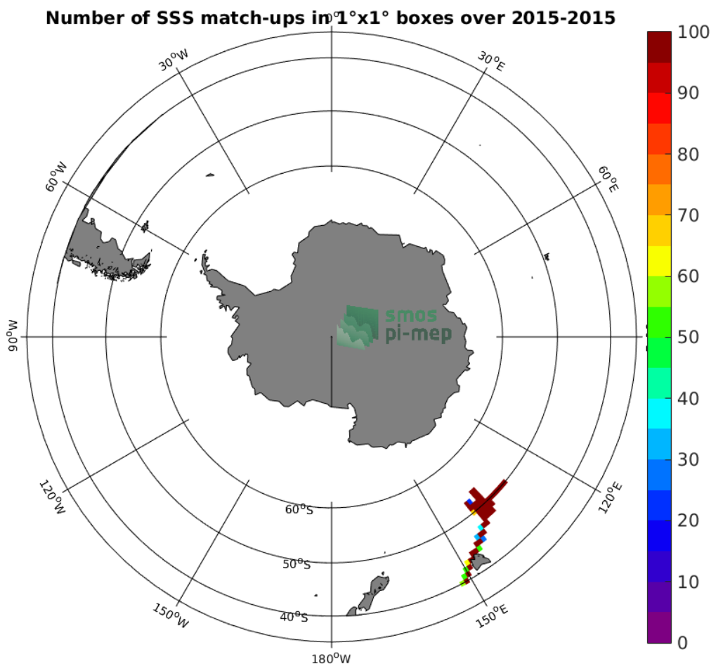
Figure 4: Number of SSS match-ups between TSG (GOSUD-Research-vessel) SSS and the SMOS L3 v2 - 9-Days (BEC) SSS product for the Roaring Forties and Furious Fifties Pi-MEP region over 1°x1° boxes and for the full satellite product period.
