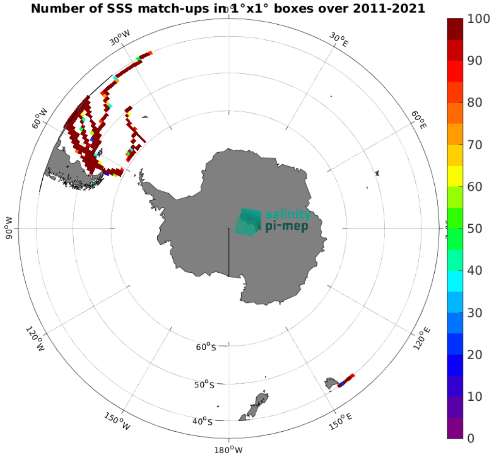
Figure 5: Number of SSS match-ups between TSG (CSIC-UTM) SSS and the SMOS SSS L3 v2 - 9-Days (BEC) SSS product for the Roaring Forties and Furious Fifties Pi-MEP region over 1^\circ \times 1^\circ boxes and for the full satellite product period.
