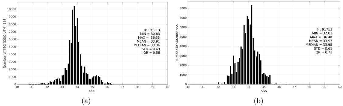
Figure 3: Histograms of SSS from TSG (CSIC-UTM) (a) and SMOS SSS L3 v2 - 9-Days (BEC) (b) considering all match-up pairs per bins of 0.1 over the Roaring Forties and Furious Fifties Pi-MEP region and for the full satellite product period.
