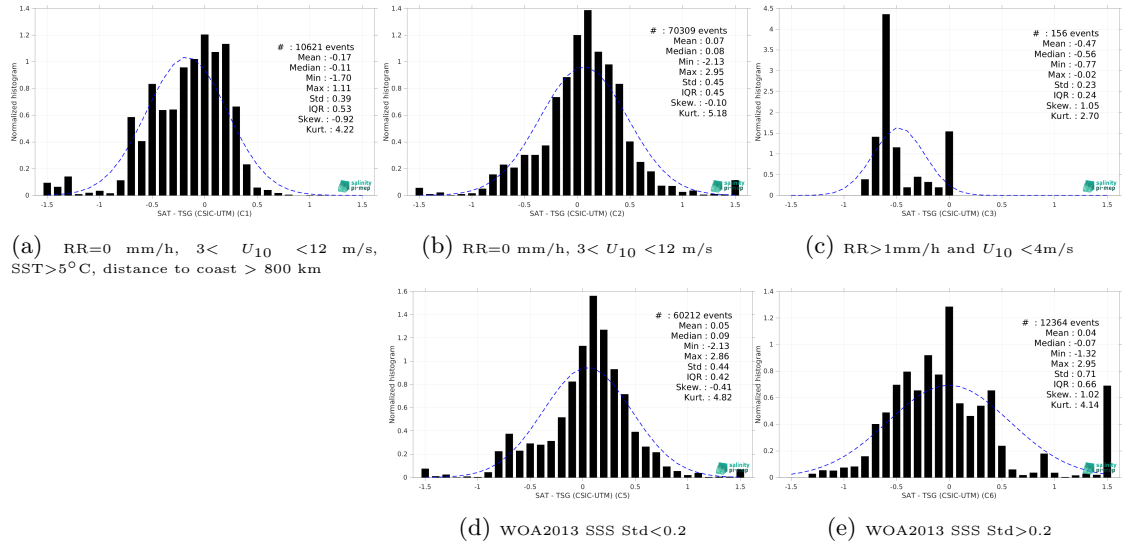
Figure 15: Normalized histogram of \Delta SSS (SMOS SSS L3 v2 - 9-Days (BEC) - TSG (CSIC-UTM)) for 5 different subdatasets corresponding to: RR=0 mm/h, 3 < U_{10} < 12 m/s, SST > 5°C, distance to coast > 800 km (a), RR=0 mm/h, 3 < U_{10} < 12 m/s (b), RR > 1mm/h and U_{10} < 4 m/s (c), WOA2013 SSS Std < 0.2 (d), WOA2013 SSS Std > 0.2 (e).
