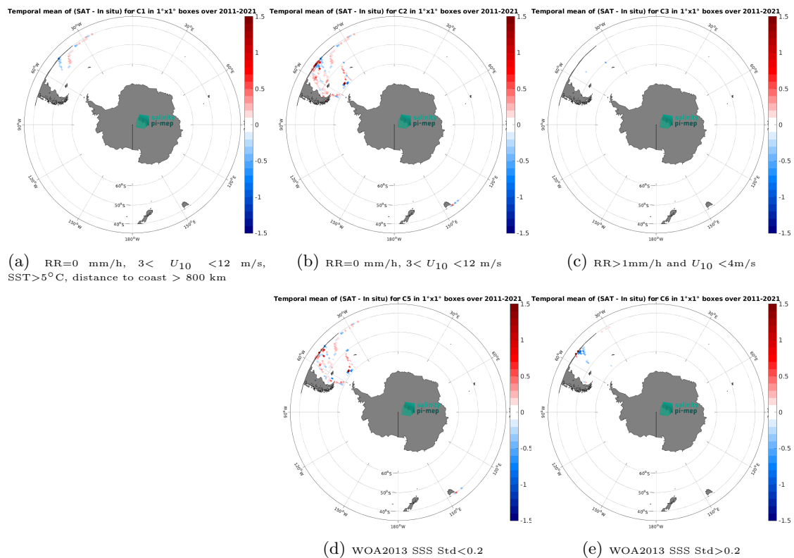
Figure 14: Temporal mean gridded over spatial boxes of size 1^\circ \times 1^\circ of \Delta SSS (SMOS SSS L3 v2 - 9-Days (BEC) - TSG (CSIC-UTM)) for 5 different subdatasets corresponding to:RR=0 mm/h, 3 < U_{10} < 12 m/s, SST > 5^\circ\text{C} , distance to coast > 800 km (a), RR=0 mm/h, 3 < U_{10} < 12 m/s (b), RR > 1 mm/h and U_{10} < 4 m/s (c), WOA2013 SSS Std < 0.2 (d), WOA2013 SSS Std > 0.2 (e).
