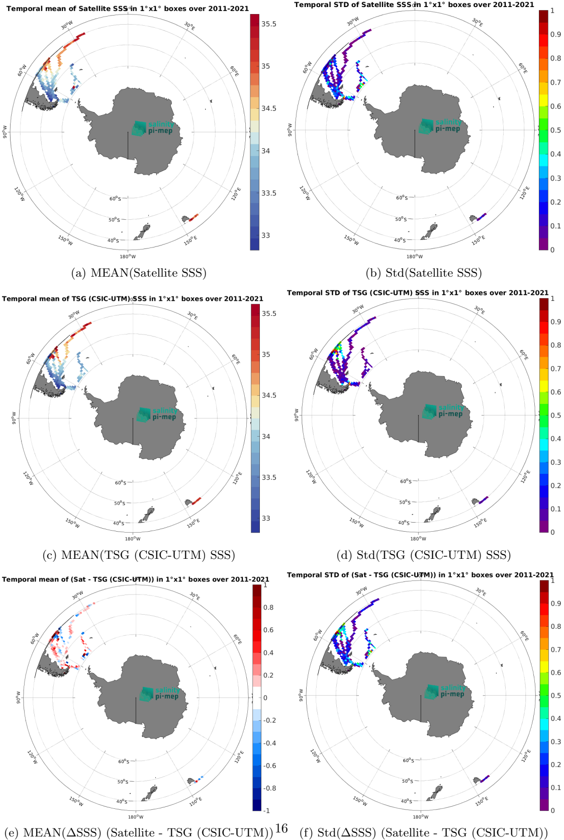
Figure 7: Temporal mean (left) and Std (right) of SSS from SMOS SSS L3 v2 - 9-Days (BEC) (top), TSG (CSIC-UTM) (middle), and of \Delta SSS (Satellite - TSG (CSIC-UTM)). Only match-up pairs are used to generate these maps.
