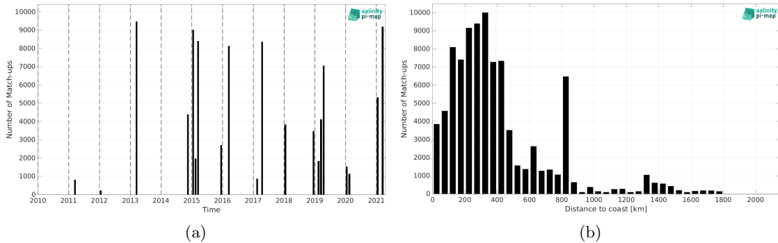
Figure 2: Number of match-ups between TSG (CSIC-UTM) and SMOS SSS L3 v2 - 9-Days (BEC) SSS as a function of time (a) and as function of the distance to coast (b) over the Roaring Forties and Furious Fifties Pi-MEP region and for the full satellite product period.
