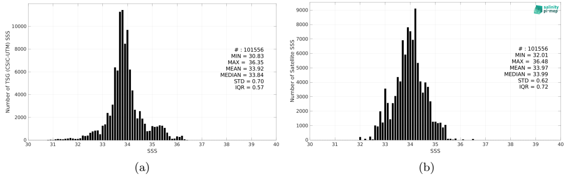
Figure 2: Histograms of SSS from TSG (CSIC-UTM) (a) and SMOS SSS L3 v2 - 9-Days (BEC) (b) considering all match-up pairs per bins of 0.1 over the Roaring Forties and Furious Fifties Pi-MEP region and for the full satellite product period.
