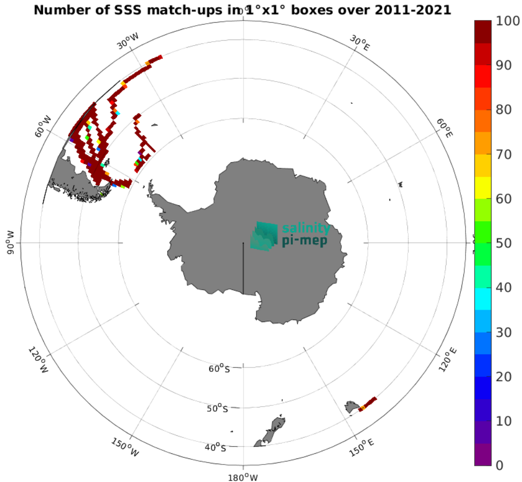
Figure 4: Number of SSS match-ups between TSG (CSIC-UTM) SSS and the SMOS SSS L3 v2 - 9-Days (BEC) SSS product for the Roaring Forties and Furious Fifties Pi-MEP region over 1^\circ \times 1^\circ boxes and for the full satellite product period.
