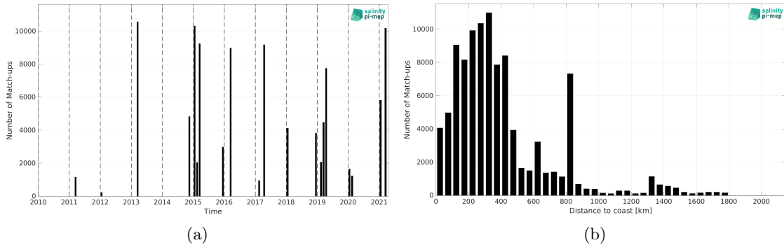
Figure 1: Number of match-ups between TSG (CSIC-UTM) and SMOS SSS L3 v2 - 9-Days (BEC) SSS as a function of time (a) and as function of the distance to coast (b) over the Roaring Forties and Furious Fifties Pi-MEP region and for the full satellite product period.
