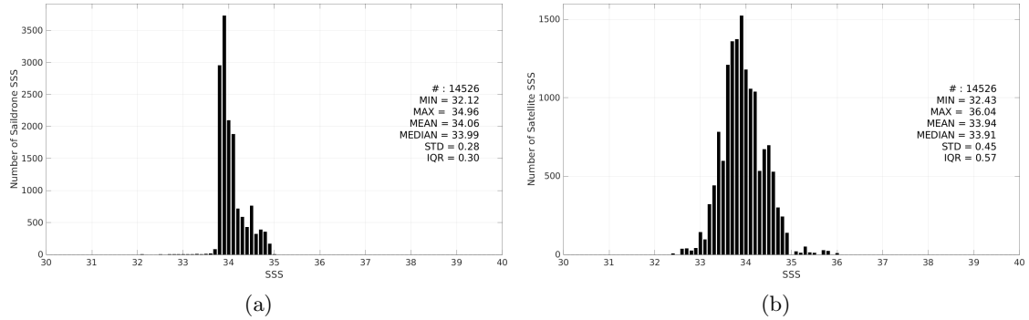
Figure 3: Histograms of SSS from Saildrone (a) and SMOS SSS L3 v2 - 9-Days (BEC) (b) considering all match-up pairs per bins of 0.1 over the Roaring Forties and Furious Fifties Pi-MEP region and for the full satellite product period.
