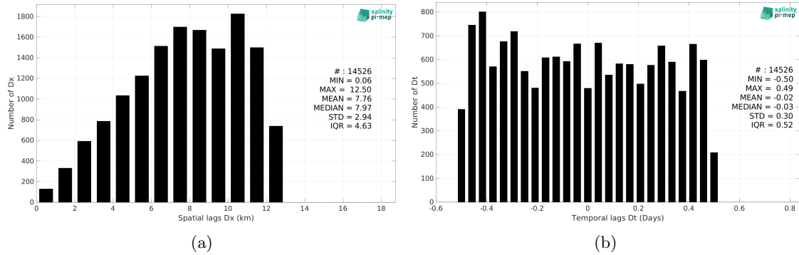
Figure 6: Histograms of the spatial (a) and temporal (b) lags between the location/time of the Saildrone measurement and the date of the corresponding SMOS SSS L3 v2 - 9-Days (BEC) SSS pixel.
