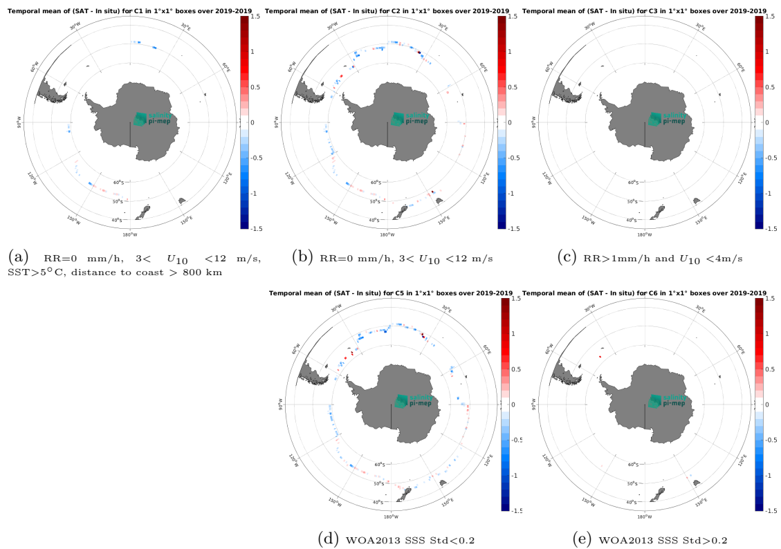
Figure 14: Temporal mean gridded over spatial boxes of size 1^\circ \times 1^\circ of \Delta SSS (SMOS SSS L3 v2 - 9-Days (BEC) - Sailydrone) for 5 different subdatasets corresponding to:RR=0 mm/h, 3 < U_{10} < 12 m/s, SST>5°C, distance to coast > 800 km (a), RR=0 mm/h, 3 < U_{10} < 12 m/s (b), RR>1mm/h and U_{10} < 4 m/s (c), WOA2013 SSS Std<0.2 (d), WOA2013 SSS Std>0.2 (e).
