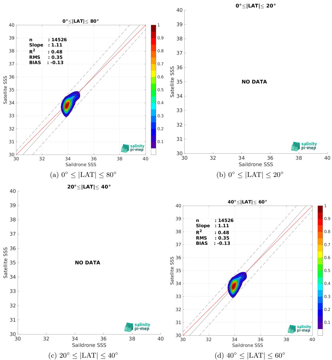
Figure 10: Contour maps of the concentration of SMOS SSS L3 v2 - 9-Days (BEC) SSS (y-axis) versus Sairdrone SSS (x-axis) at match-up pairs for different latitude bands. For each plot, the red line shows x=y . The black thin and dashed lines indicate a linear fit through the data cloud and the \pm 95\% confidence levels, respectively. The number match-up pairs n , the slope and R^2 coefficient of the linear fit, the root mean square (RMS) and the mean bias between satellite and in situ data are indicated for each latitude band in each plots.
