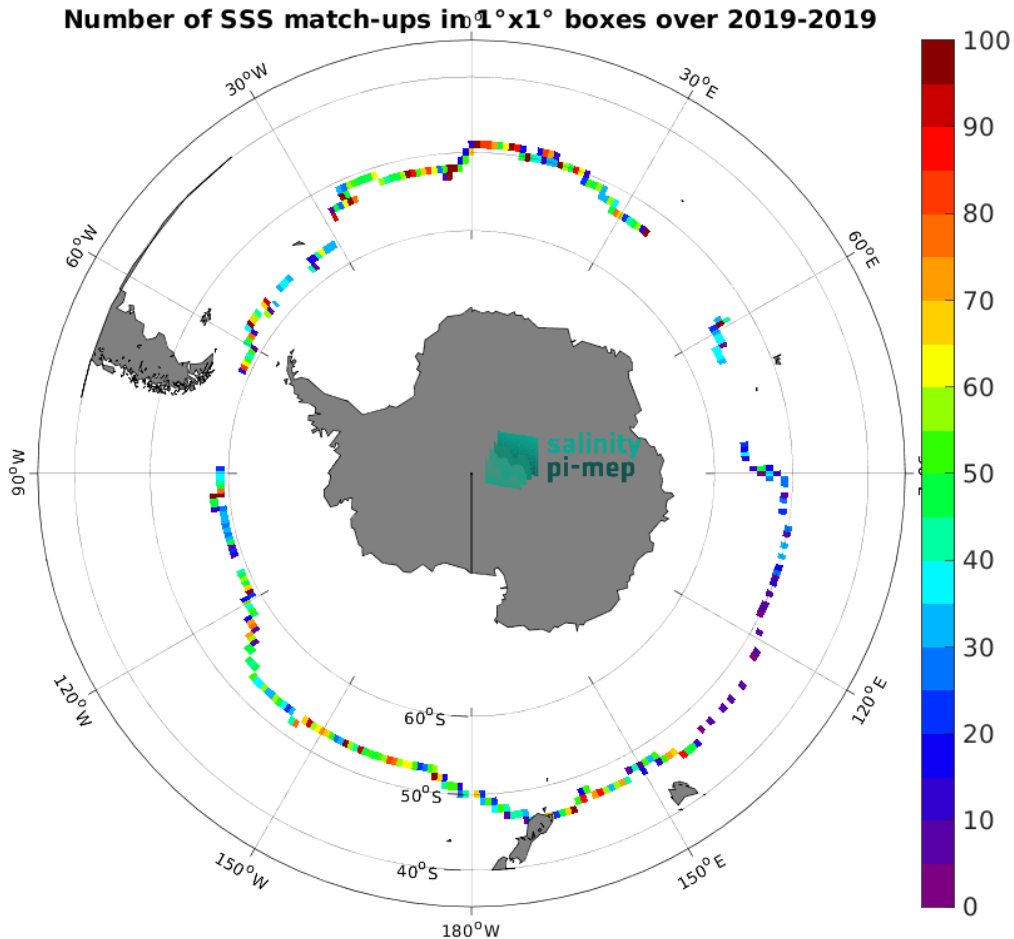
Figure 5: Number of SSS match-ups between Saildrone SSS and the SMOS SSS L3 v2 - 9-Days (BEC) SSS product for the Roaring Forties and Furious Fifties Pi-MEP region over 1^\circ \times 1^\circ boxes and for the full satellite product period.
