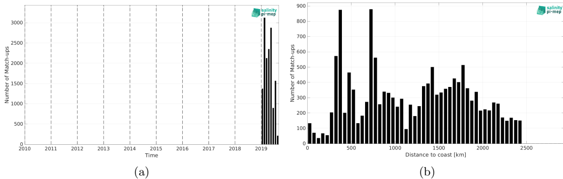
Figure 2: Number of match-ups between Saildrone and SMOS SSS L3 v2 - 9-Days (BEC) SSS as a function of time (a) and as function of the distance to coast (b) over the Roaring Forties and Furious Fifties Pi-MEP region and for the full satellite product period.
