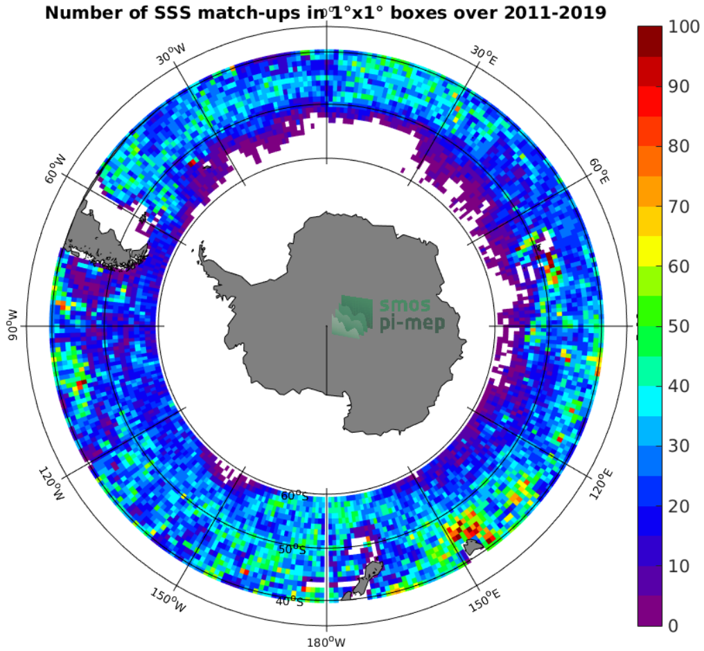
Figure 4: Number of SSS match-ups between Argo SSS and the SMOS SSS L3 v2 - 9-Days (BEC) SSS product for the Roaring Forties and Furious Fifties Pi-MEP region over 1^\circ \times 1^\circ boxes and for the full satellite product period.
