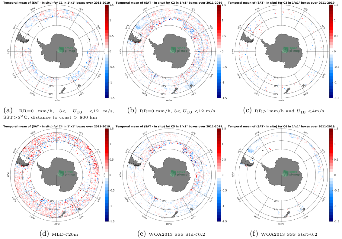
Figure 12: Temporal mean gridded over spatial boxes of size 1^{\circ} \times 1^{\circ} of \Delta\text{SSS} (SMOS SSS L3 v2 - 9-Days (BEC) - Argo) for 6 different subdatasets corresponding to: \text{RR}=0 mm/h, 3 < U_{10} < 12 m/s, \text{SST} > 5^{\circ}\text{C} , distance to coast > 800 km (a), \text{RR}=0 mm/h, 3 < U_{10} < 12 m/s (b), \text{RR} > 1\text{mm/h} and U_{10} < 4\text{m/s} (c), \text{MLD} < 20\text{m} (d), \text{WOA2013 SSS Std} < 0.2 (e), \text{WOA2013 SSS Std} > 0.2 (f).
