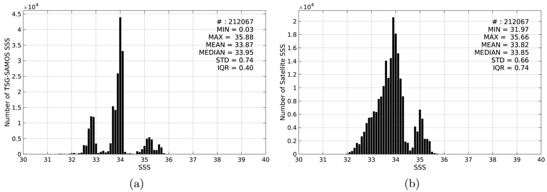
Figure 2: Histograms of SSS from TSG-SAMOS (a) and SMOS-L3-BEC-OA-V1-9DAYS-0.25DEG (b) considering all match-up pairs per bins of 0.1 over the Roaring Forties and Furious Fifties Pi-MEP region and for the full satellite product period.
