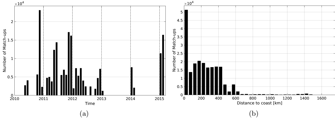
Figure 1: Number of match-ups between TSG-SAMOS and SMOS-L3-BEC-OA-V1-9DAYS-0.25DEG SSS as a function of time (a) and as function of the distance to coast (b) over the Roaring Forties and Furious Fifties Pi-MEP region and for the full satellite product period.
