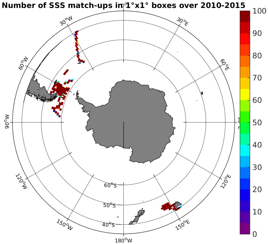
Figure 4: Number of SSS match-ups between TSG-SAMOS SSS and the SMOS-L3-BEC-OA-V1-9DAYS-0.25DEG SSS product for the Roaring Forties and Furious Fifties Pi-MEP region over 1°x1° boxes and for the full satellite product period.
