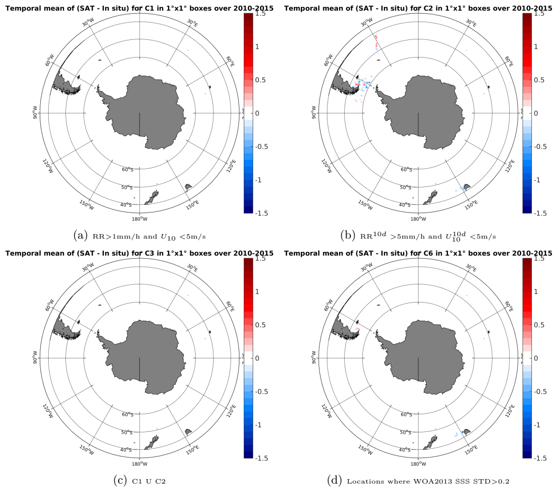
Figure 12: Temporal mean gridded over spatial boxes of size 1^\circ \times 1^\circ of \Delta SSS (SMOS-L3-BEC-OA-V1-9DAYS-0.25DEG - TSG-SAMOS) for 4 different subdatasets corresponding to: RR > 1\text{mm/h} and U_{10} < 5\text{m/s} (a), RR^{10d} > 5\text{mm/h} and U_{10}^{10d} < 5\text{m/s} (b), C1 U C2 (c), Locations where WOA2013 SSS STD > 0.2 (d).
