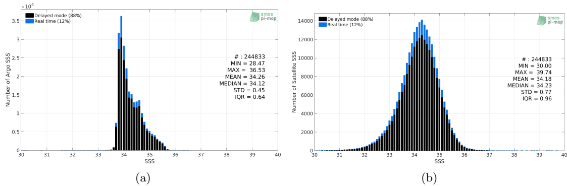
Figure 2: Histograms of SSS from Argo (a) and SMOS SSS L2-AVERAGED v700 (ESA) (b) considering all match-up pairs per bins of 0.1 over the Roaring Forties and Furious Fifties Pi-MEP region and for the full satellite product period.
