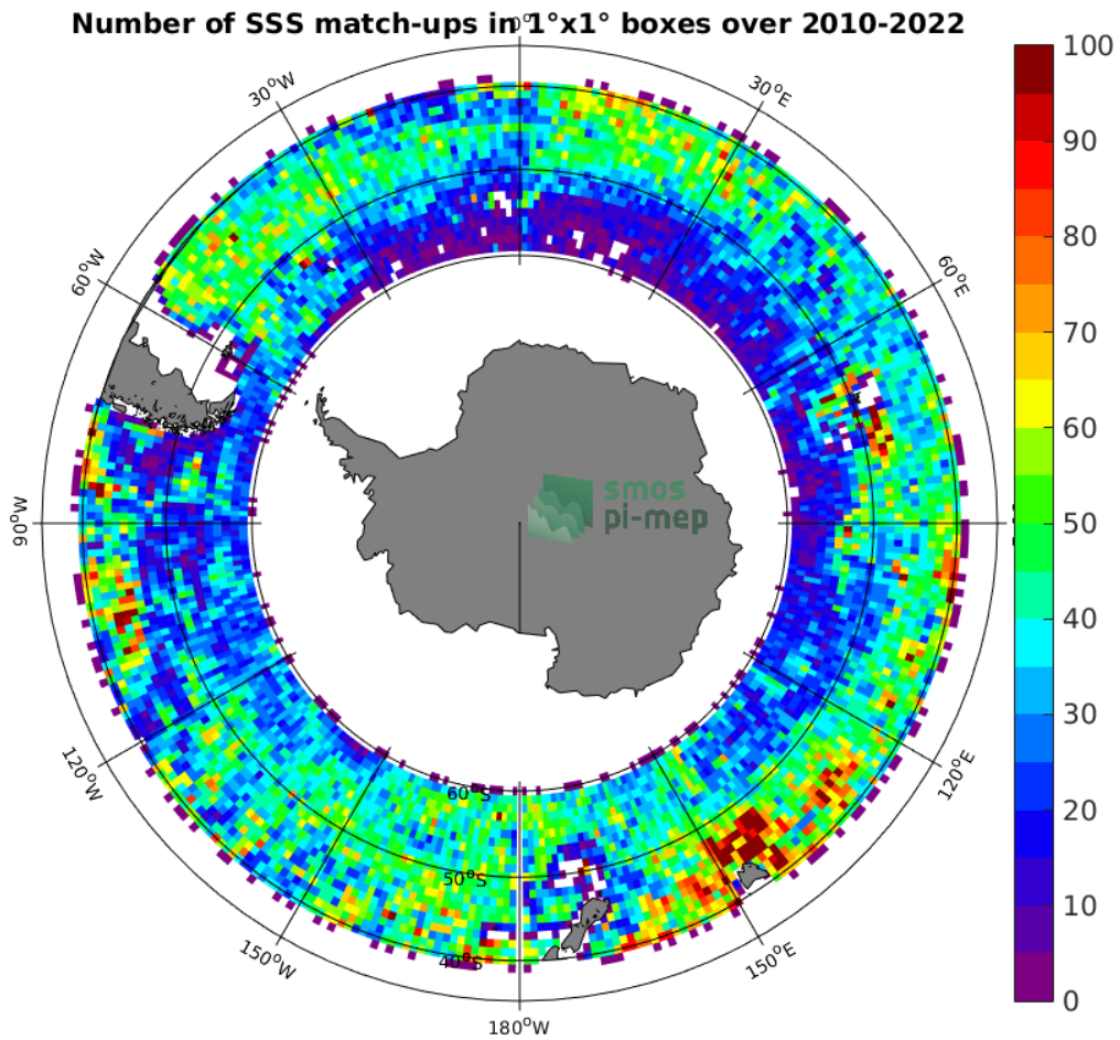
Figure 4: Number of SSS match-ups between Argo SSS and the SMOS SSS L2-AVERAGED v700 (ESA) SSS product for the Roaring Forties and Furious Fifties Pi-MEP region over 1^\circ \times 1^\circ boxes and for the full satellite product period.
