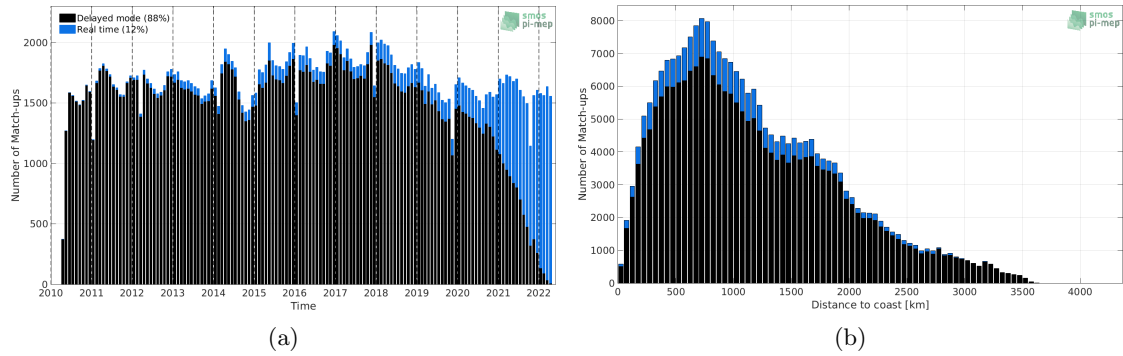
Figure 1: Number of match-ups between Argo and SMOS SSS L2-AVERAGED v700 (ESA) SSS as a function of time (a) and as function of the distance to coast (b) over the Roaring Forties and Furious Fifties Pi-MEP region and for the full satellite product period.
