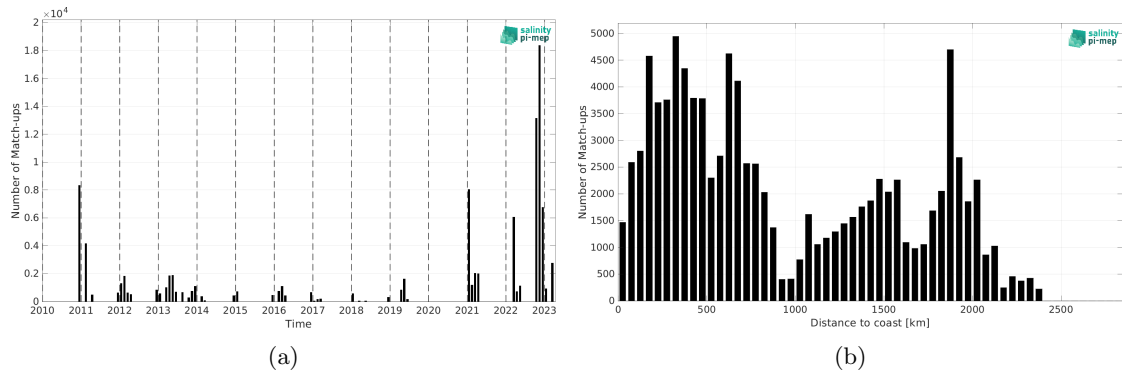
Figure 2: Number of match-ups between TSG (Polarstern) and SMOS SSS L2 v700 (ESA) SSS as a function of time (a) and as function of the distance to coast (b) over the Roaring Forties and Furious Fifties Pi-MEP region and for the full satellite product period.
