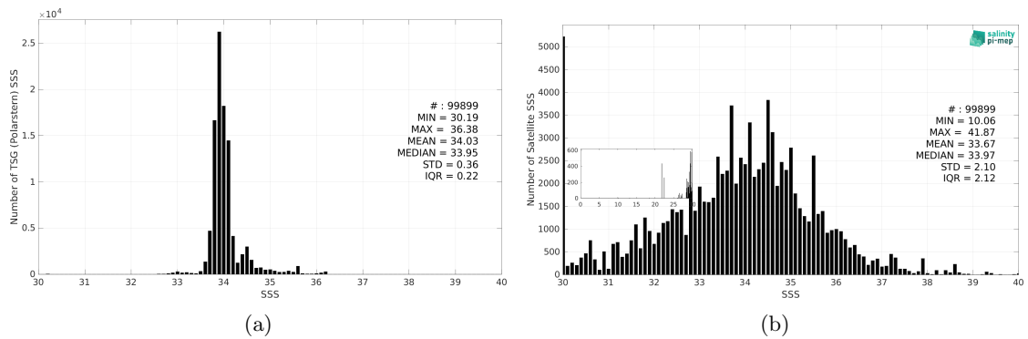
Figure 3: Histograms of SSS from TSG (Polarstern) (a) and SMOS SSS L2 v700 (ESA) (b) considering all match-up pairs per bins of 0.1 over the Roaring Forties and Furious Fifties Pi-MEP region and for the full satellite product period.
