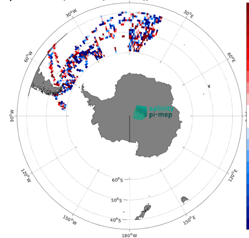
(e) MEAN( \Delta SSS) (Satellite - TSG (Polarstern)) 20
