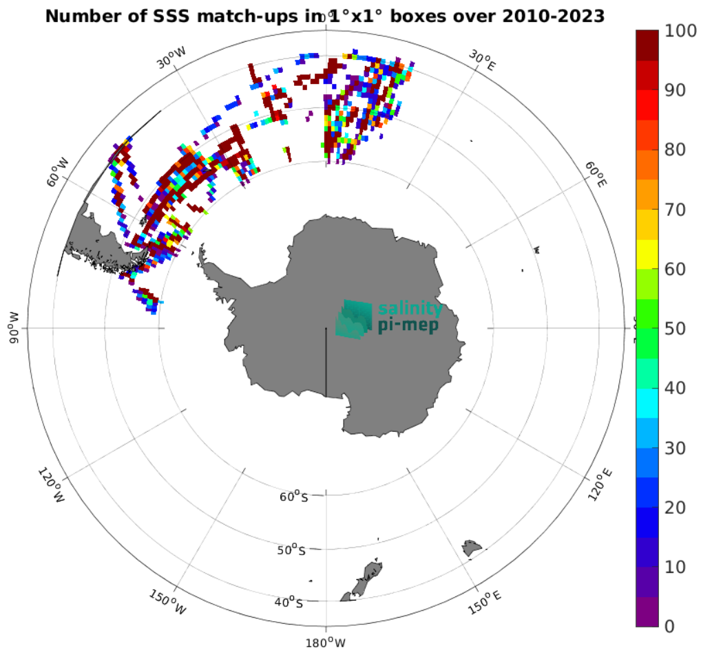
Figure 5: Number of SSS match-ups between TSG (Polarstern) SSS and the SMOS SSS L2 v700 (ESA) SSS product for the Roaring Forties and Furious Fifties Pi-MEP region over 1^\circ \times 1^\circ boxes and for the full satellite product period.
