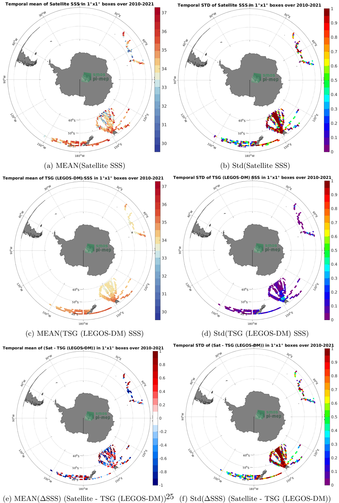
Figure 6: Temporal mean (left) and Std (right) of SSS from SMOS SSS L2 v700 (ESA) (top), TSG (LEGOS-DM) (middle), and of \Delta SSS (Satellite - TSG (LEGOS-DM)). Only match-up pairs are used to generate these maps.
