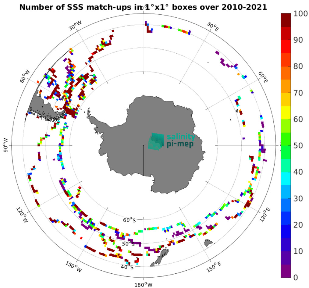
Figure 5: Number of SSS match-ups between TSG (GOSUD-Sailing-ship) SSS and the SMOS SSS L2 v700 (ESA) SSS product for the Roaring Forties and Furious Fifties Pi-MEP region over 1^\circ \times 1^\circ boxes and for the full satellite product period.
