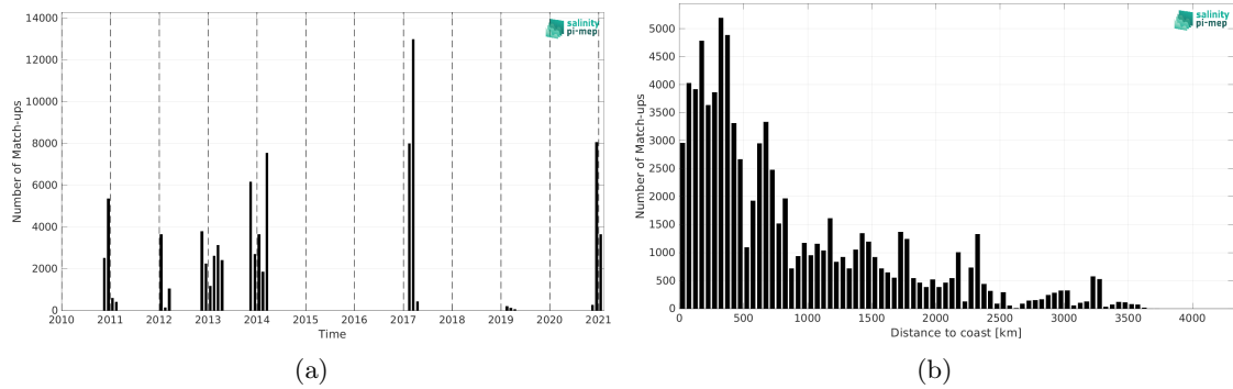
Figure 2: Number of match-ups between TSG (GOSUD-Sailing-ship) and SMOS SSS L2 v700 (ESA) SSS as a function of time (a) and as function of the distance to coast (b) over the Roaring Forties and Furious Fifties Pi-MEP region and for the full satellite product period.
