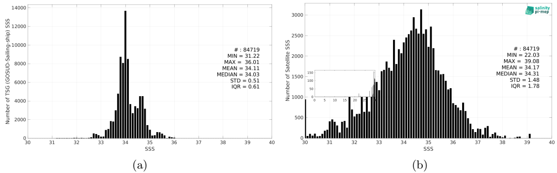
Figure 3: Histograms of SSS from TSG (GOSUD-Sailing-ship) (a) and SMOS SSS L2 v700 (ESA) (b) considering all match-up pairs per bins of 0.1 over the Roaring Forties and Furious Fifties Pi-MEP region and for the full satellite product period.
