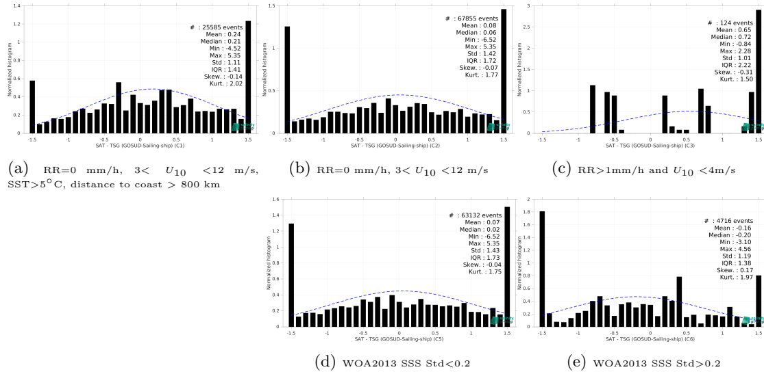
Figure 15: Normalized histogram of \Delta SSS (SMOS SSS L2 v700 (ESA) - TSG (GOSUD-Sailing-ship)) for 5 different subdatasets corresponding to: RR=0 mm/h, 3 < U_{10} < 12 m/s, SST >5^{\circ} C, distance to coast > 800 km (a), RR=0 mm/h, 3 < U_{10} < 12 m/s (b), RR >1 mm/h and U_{10} < 4 m/s (c), WOA2013 SSS Std <0.2 (d), WOA2013 SSS Std >0.2 (e).
