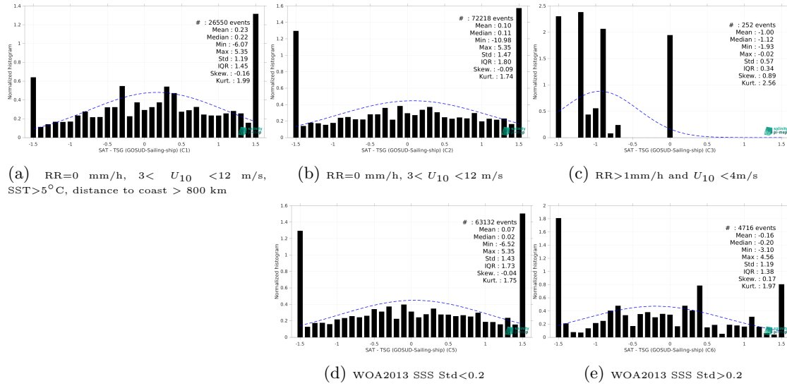
Figure 13: Normalized histogram of \Delta\text{SSS} (SMOS SSS L2 v700 (ESA) - TSG (GOSUD-Sailing-ship)) for 5 different subdatasets corresponding to: RR=0 mm/h, 3 < U_{10} < 12 m/s, SST>5°C, distance to coast > 800 km (a), RR=0 mm/h, 3 < U_{10} < 12 m/s (b), RR>1mm/h and U_{10} < 4 m/s (c), WOA2013 SSS Std<0.2 (d), WOA2013 SSS Std>0.2 (e).
