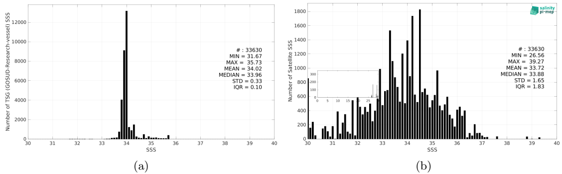
Figure 3: Histograms of SSS from TSG (GOSUD-Research-vessel) (a) and SMOS SSS L2 v700 (ESA) (b) considering all match-up pairs per bins of 0.1 over the Roaring Forties and Furious Fifties Pi-MEP region and for the full satellite product period.
