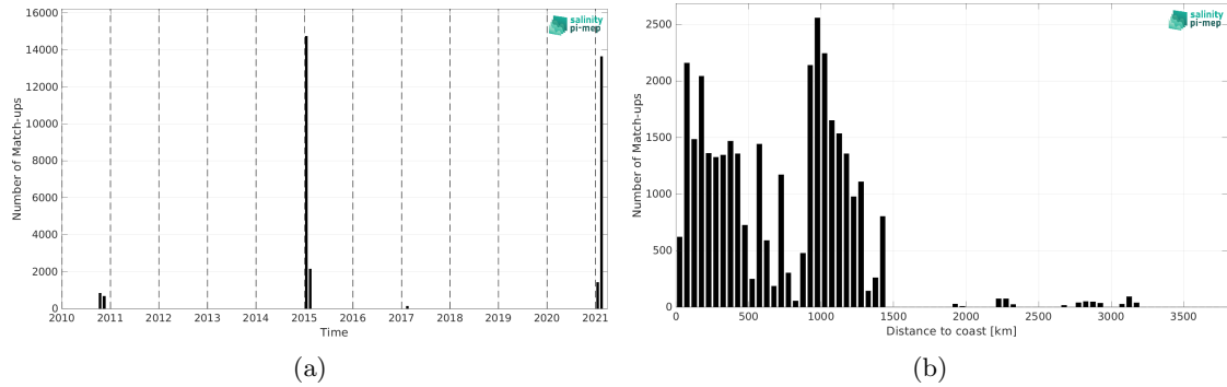
Figure 2: Number of match-ups between TSG (GOSUD-Research-vessel) and SMOS SSS L2 v700 (ESA) SSS as a function of time (a) and as function of the distance to coast (b) over the Roaring Forties and Furious Fifties Pi-MEP region and for the full satellite product period.
