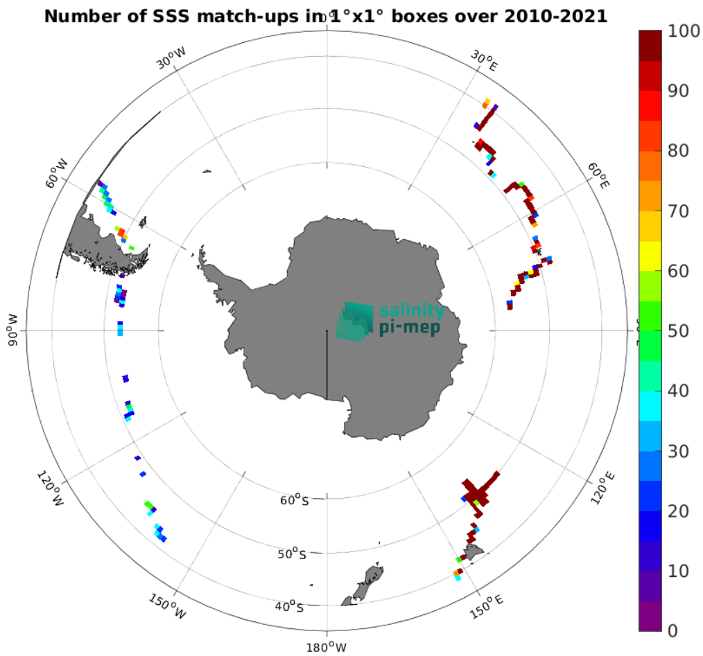
Figure 5: Number of SSS match-ups between TSG (GOSUD-Research-vessel) SSS and the SMOS SSS L2 v700 (ESA) SSS product for the Roaring Forties and Furious Fifties Pi-MEP region over 1^\circ \times 1^\circ boxes and for the full satellite product period.
