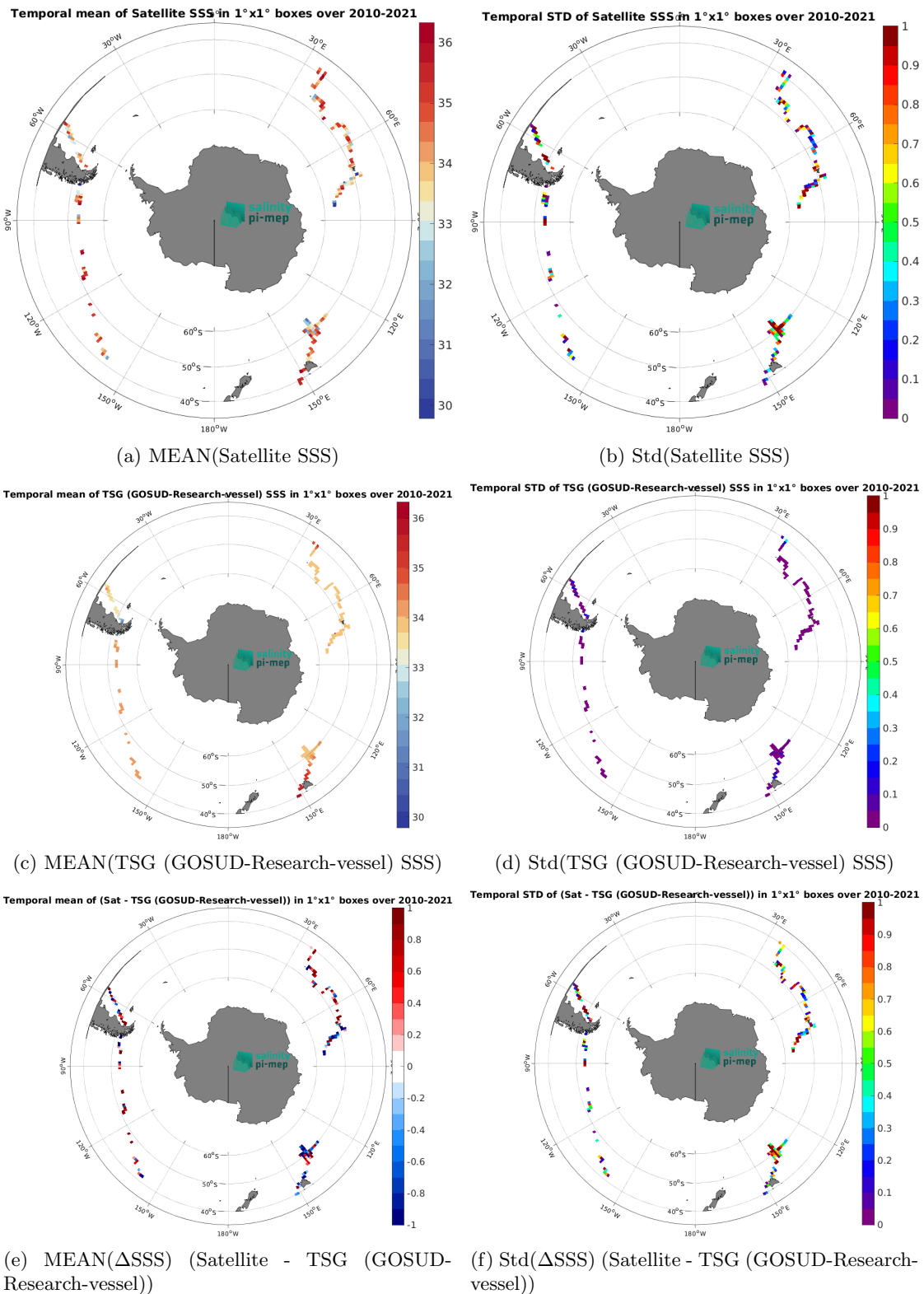
Figure 7: Temporal mean (left) and Std (right) of SSS from SMOS SSS L2 v700 (ESA) (top), TSG (GOSUD-Research-vessel) (middle), and of \Delta SSS (Satellite - TSG (GOSUD-Research-vessel)). Only match-up pairs are used to generate these maps.
