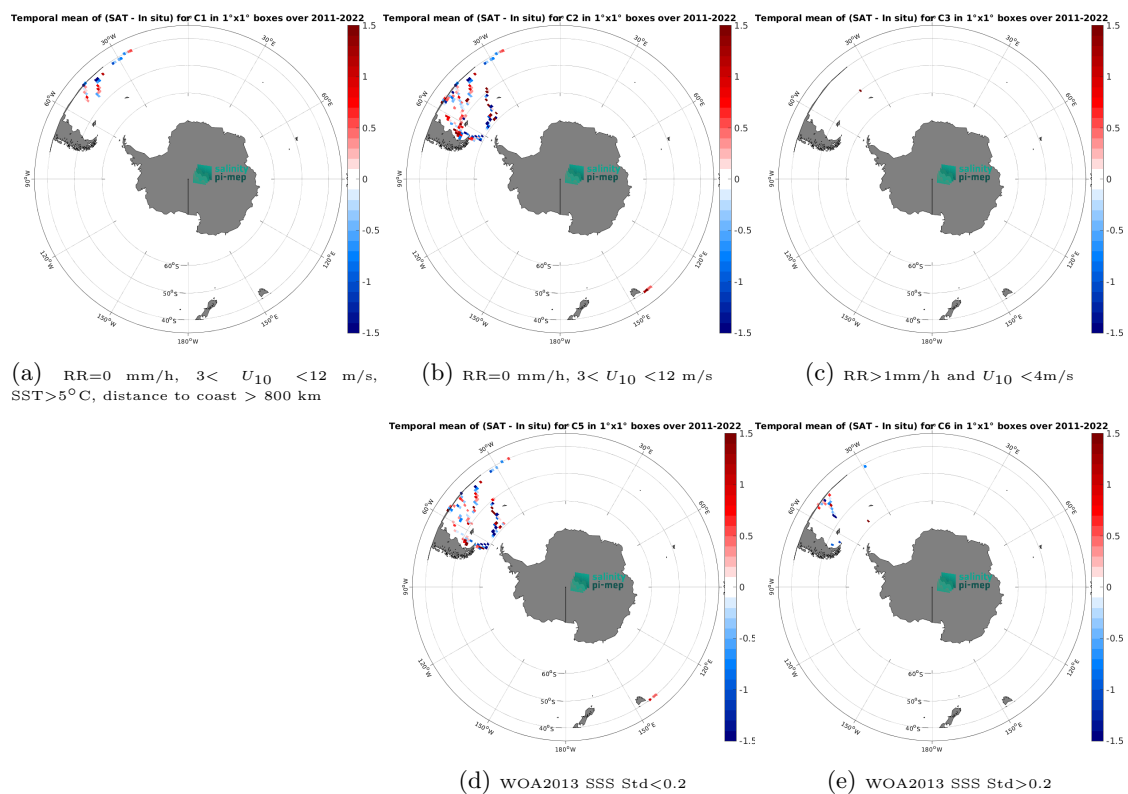
Figure 14: Temporal mean gridded over spatial boxes of size 1^\circ \times 1^\circ of \Delta SSS (SMOS SSS L2 v700 (ESA) - TSG (CSIC-UTM)) for 5 different subdatasets corresponding to:RR=0 mm/h, 3 < U_{10} < 12 m/s, SST>5°C, distance to coast > 800 km (a), RR=0 mm/h, 3 < U_{10} < 12 m/s (b), RR>1mm/h and U_{10} < 4 m/s (c), WOA2013 SSS Std<0.2 (d), WOA2013 SSS Std>0.2 (e).
