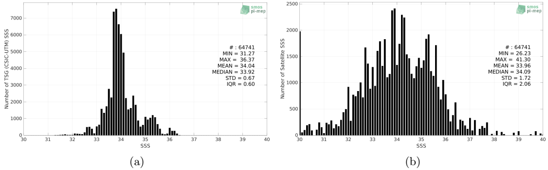
Figure 2: Histograms of SSS from TSG (CSIC-UTM) (a) and SMOS SSS L2 v700 (ESA) (b) considering all match-up pairs per bins of 0.1 over the Roaring Forties and Furious Fifties Pi-MEP region and for the full satellite product period.
