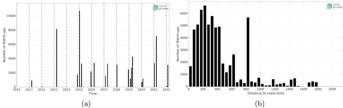
Figure 1: Number of match-ups between TSG (CSIC-UTM) and SMOS SSS L2 v700 (ESA) SSS as a function of time (a) and as function of the distance to coast (b) over the Roaring Forties and Furious Fifties Pi-MEP region and for the full satellite product period.
