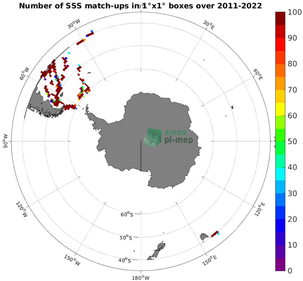
Figure 4: Number of SSS match-ups between TSG (CSIC-UTM) SSS and the SMOS SSS L2 v700 (ESA) SSS product for the Roaring Forties and Furious Fifties Pi-MEP region over 1^\circ \times 1^\circ boxes and for the full satellite product period.
