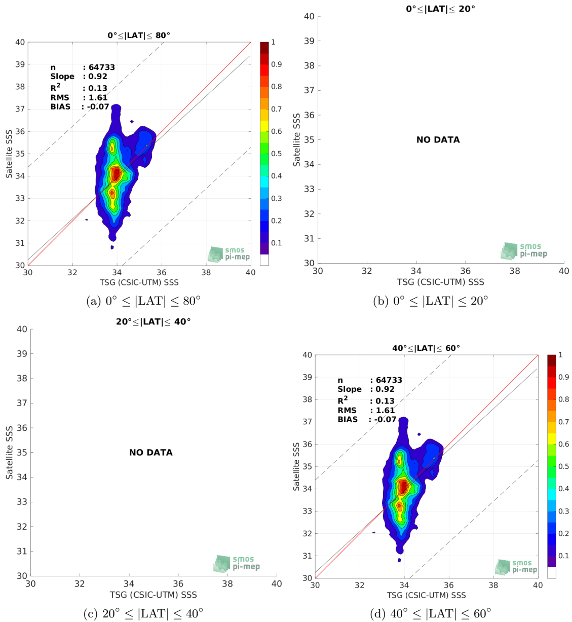
Figure 9: Contour maps of the concentration of SMOS SSS L2 v700 (ESA) SSS (y-axis) versus TSG (CSIC-UTM) SSS (x-axis) at match-up pairs for different latitude bands. For each plot, the red line shows x=y . The black thin and dashed lines indicate a linear fit through the data cloud and the \pm 95\% confidence levels, respectively. The number match-up pairs n , the slope and R^2 coefficient of the linear fit, the root mean square (RMS) and the mean bias between satellite and in situ data are indicated for each latitude band in each plot.
