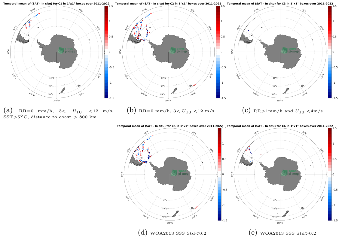
Figure 12: Temporal mean gridded over spatial boxes of size 1^{\circ}\times 1^{\circ} of \Delta\text{SSS} (SMOS SSS L2 v700 (ESA) - TSG (CSIC-UTM)) for 5 different subdatasets corresponding to: \text{RR}=0 mm/h, 3 < U_{10} < 12 m/s, \text{SST}>5^{\circ}\text{C} , distance to coast > 800 km (a), \text{RR}=0 mm/h, 3 < U_{10} < 12 m/s (b), \text{RR}>1 mm/h and U_{10} < 4 m/s (c), WOA2013 SSS Std < 0.2 (d), WOA2013 SSS Std > 0.2 (e).
