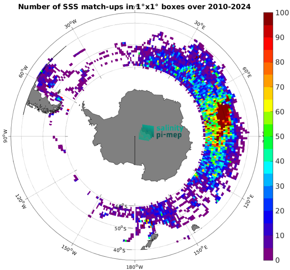
Figure 5: Number of SSS match-ups between Marine mammals SSS and the SMOS SSS L2 v700 (ESA) SSS product for the Roaring Forties and Furious Fifties Pi-MEP region over 1^{\circ} \times 1^{\circ} boxes and for the full satellite product period.
